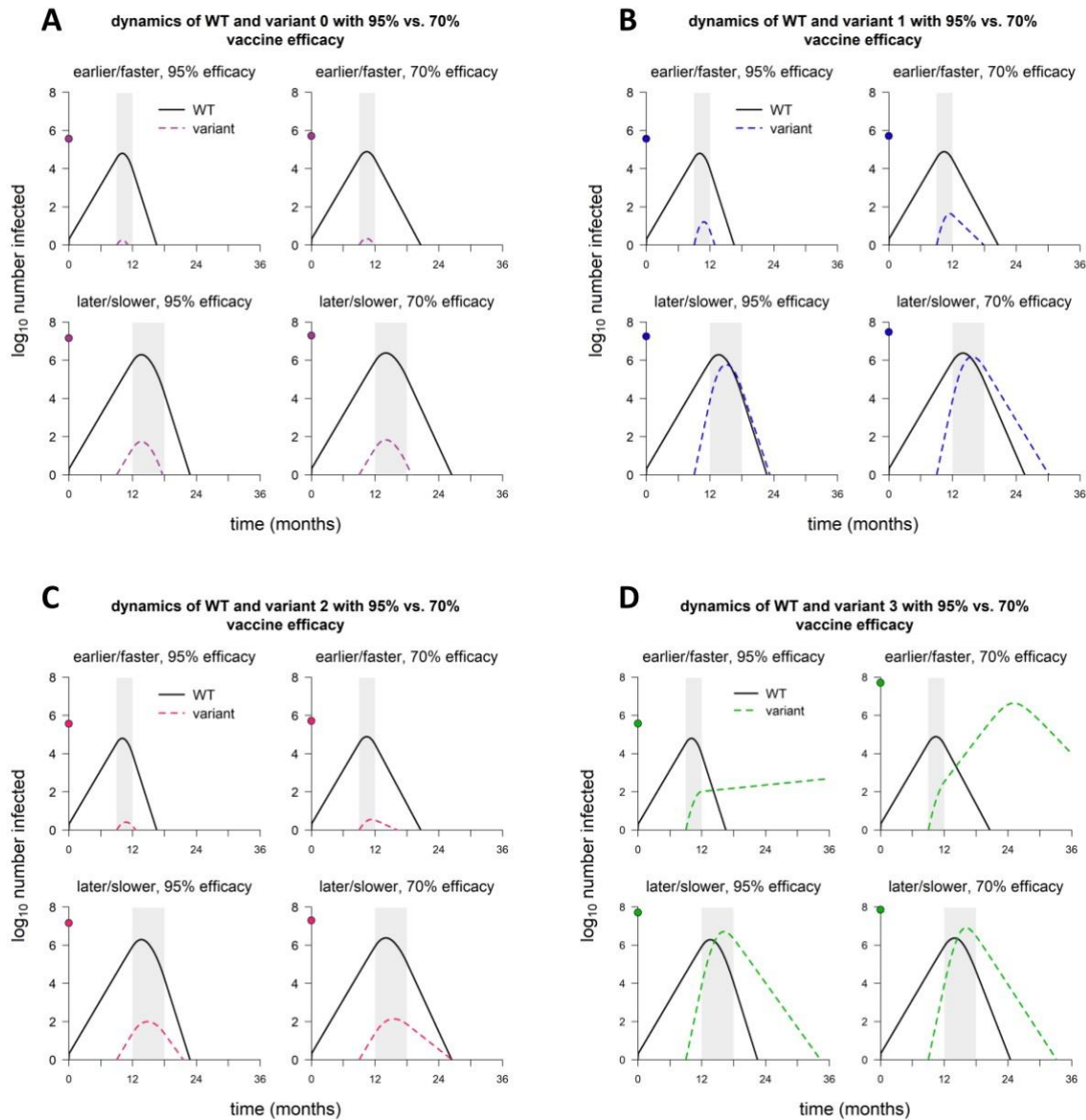
Fig S3. Dynamics of WT and variant strains with rapid vs. delayed vaccine rollout and 95% baseline vaccine efficacy vs. 70% baseline efficacy. (A) Dynamics of WT and variant 0. (B) WT and variant 1. (C) WT and variant 2. (D) WT and variant 3. Simulation conditions as follows: earlier/faster vaccine rollout = starting at 9 months and lasting 3 months; later/slower rollout = starting at 12 months and lasting 6 months. Variant introduced at 9 months in all simulations. Solid/black lines, WT; colored/dashed lines, variants; gray shading, vaccine rollout. In each panel, point on y-axis indicates total number of infections over the entire simulation. Variant phenotypes are as follows: variant 0, identical to WT; variant 1, 60% greater transmissibility; variant 2, 40% immune escape; variant 3, 60% greater transmissibility and 40% immune escape.
