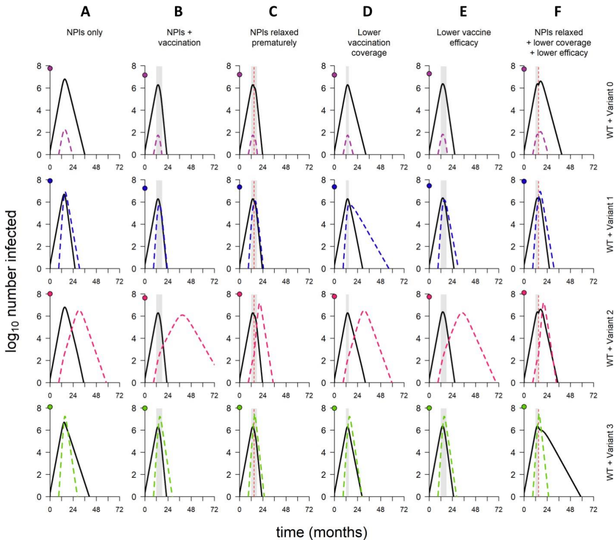
Fig S11. Dynamics of WT and variants, in simulations with varying combinations of control measures, for alternative model with higher degree of immune escape. (A) No vaccination but NPIs in place throughout. (B) Default model conditions (NPIs in place throughout, 100% vaccination coverage, 95% vaccine efficacy against WT). (C) NPIs lifted when vaccination coverage reaches 50% (other model conditions as in B). (D) 50% vaccination coverage (other model conditions as in B). (E) 70% vaccine efficacy (other model conditions as in B). (F) Combination of conditions C through E (NPIs relaxed, 50% vaccination coverage, and 70% vaccine efficacy). In each panel, point on y-axis indicates the total number of infections over the entire simulation. All simulations run for an extended duration of six years (default condition is three years); variant introduced at 9 months; in simulations with vaccination, rollout begins at 12 months and lasts 6 months if final coverage is 100%, 3 months if final coverage is 50%. Solid/black lines, WT; colored/dashed lines, variants; gray shading, vaccine rollout; dashed vertical line, 50% vaccination coverage. Variant phenotypes are as follows: variant 0, identical to WT; variant 1,
