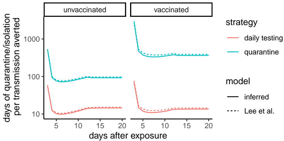
Supplementary Figure 5: Cost-benefit ratio for quarantine strategy and DCT strategy for vaccinated and unvaccinated contacts. The cost-benefit ratio is defined as the total days of quarantine or self-isolation per transmission averted. Results using the relationship between viral load and infectiousness inferred in this paper are shown as solid lines; results using the relationship inferred by Lee et al are shown as dashed lines.
