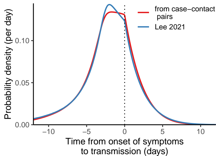
Supplementary Figure 3: Distribution of the time from onset of symptoms to transmission (TOST), according to the two different relationships between infectiousness and viral load discussed in the text.
