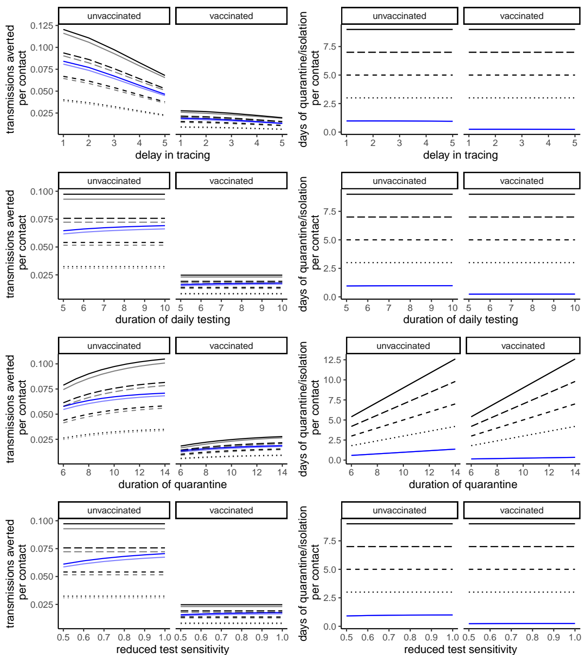
Supplementary Figure 6: Total number of transmissions averted by quarantine or DCT strategies for contact-traced individuals, and number of days of quarantine per traced individual. Quarantine is shown as black lines; daily testing is shown in blue. Solid lines correspond to inference of infectiousness from timing of transmission of case-contact pairs, semi-transparent lines to inference from Lee et al. Each row explores a different range for a given parameter with respect to the default scenario in Figure 3.
