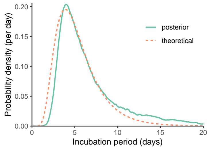
Supplementary Figure 1: Theoretical distribution of the incubation period used in the likelihood (orange dashed line), and simulated empirical distribution for the incubation period obtained from the inferred model (green solid line).
