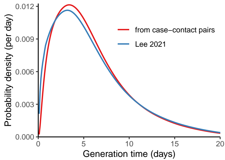
Supplementary Figure 2: Distribution of the generation time (the time from becoming infected oneself to infecting others), according to the two different relationships between infectiousness and viral load discussed in the text.
