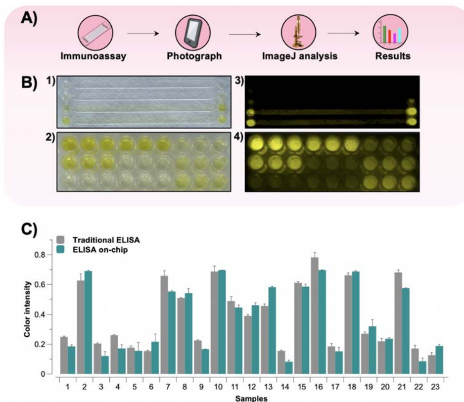
Figure 4. A) Analysis methodology: First, the immunoassay is performed. Then, a photograph of the substrate, either a microplate or a microfluidic device, is acquired with a smartphone, followed by a color intensity analysis of the resulting colorimetric reactions using the ImageJ software or any other similar software. Finally, the results are plotted and compared against the ones obtained from other samples. B) Photographs of the resulting reactions when
