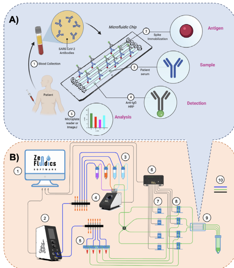
Figure 1. Assay's methodology and experimental setup. A) The methodology followed in our automated ELISA on-chip assay included the steps listed below: 1) Blood collection and serum extraction, 2) On-chip immobilization of viral antigens (SARS-CoV-2 spike protein), 3) Pumping serum samples through the microfluidic device (if present, anti-SARS-CoV-2 antibodies interact with the immobilized SARS-CoV-2 spike proteins), 4) Pumping anti-IgG-HRP through the micro-fluidic device to detect IgG antibodies, and 5) Analysis of the colorimetric reaction, either by recovering the resulting reaction and performing the analysis with a microplate reader or by carrying out a color intensity analysis using ImageJ software. B) Diagram of the experimental setup assembled for our automated ELISA on-chip. The components are listed below: 1) Software that controls all the peripheral devices of the setup, 2) Flow control unit, 3) ELISA reagents (wash buffer, blocking buffer, and anti-IgG-HRP conjugate antibody), 4) 12/1 bidirectional microfluidic rotary valve, 5) Serum samples, 6) Microfluidic valve controller, 7) Pinch valves, 8) 3/2-way switching valves, 9) Microfluidic device, and 10) Connections between components and reservoirs (color code: blue is for pneumatic connections, green is for fluid connections, and black is for electrical connections).
