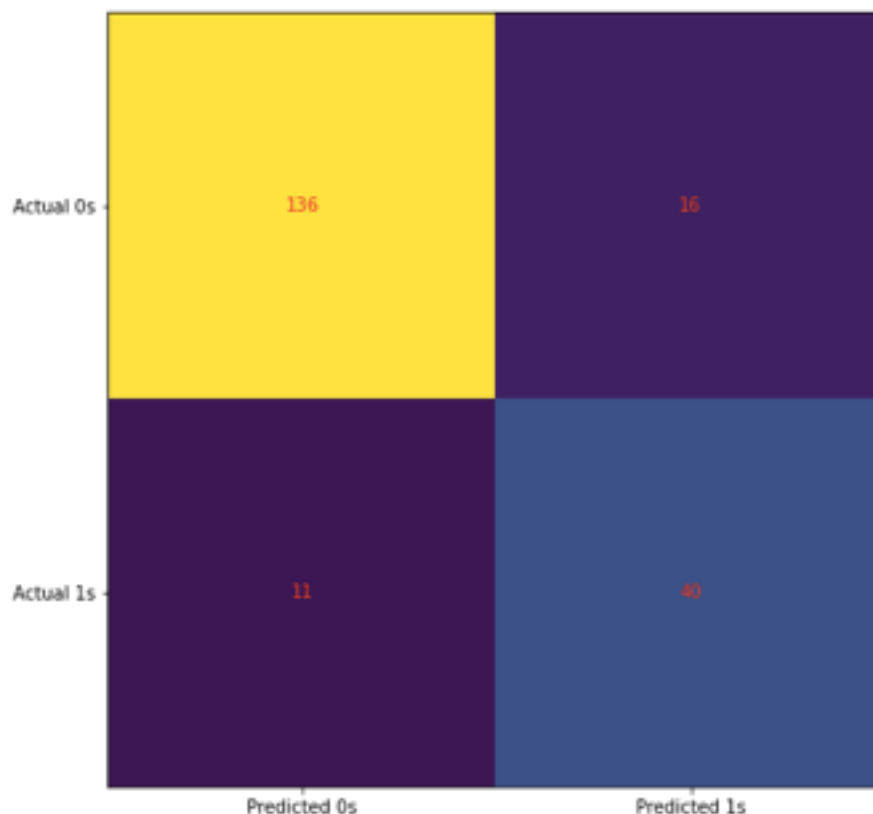
Figure 1: Confusion matrix for model 1
