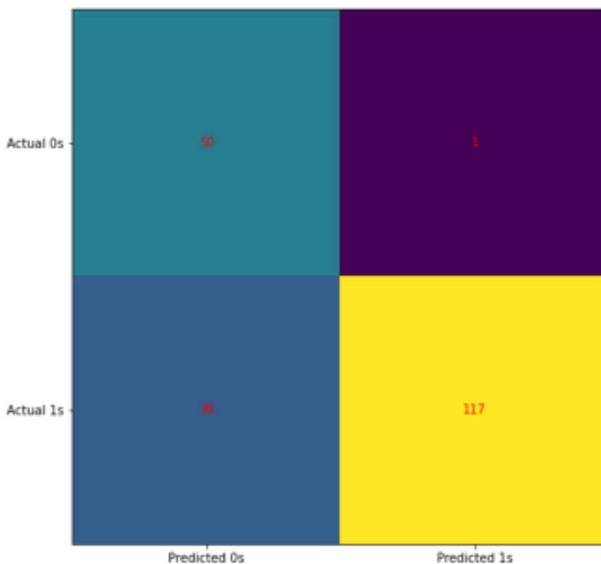
Figure 2: Confusion matrix for model 2
