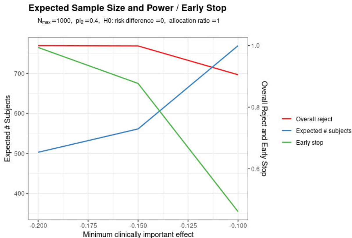
Figure 1. Plot of average expected sample size and power for a Wang & Tsiatis design with two looks. 3 Minimum clinically important effect of 0.2, 0.15, or 0.1, derived for a DGE rate \pi_1 = \{0.2, 0.25, 0.3\} in the experimental group (prPD). \pi_2 = 0.4 depicts the DGE rate in the reference group (ppPD). ppPD = Pylorus preservation in pancreaticoduodenectomy; prPD = Pylorus resection in pancreaticoduodenectomy.
