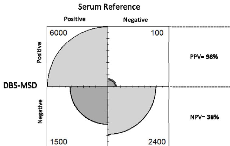
Figure 3: Confusion matrix showing the predictive performance of MSD-DBS in a theoretical population (n=10,000) with seventy-five percent SARS-CoV-2 vaccine coverage. The positive-predictive value (PPV) of MSD-DBS is positively correlated with the prevalence of SARS-CoV-2 seroreactivity. At seventy-five percent SARS-CoV-2 vaccine coverage, a positive MSD-DBS test would correctly identify vaccine elicited seroreactivity at a 98% rate, PPV= 98% (95% CI: 98%-99%). A negative MSD-DBS test correctly identifies no vaccine elicited seroreactivity at a 38% rate, negative predictive value (NPV)= 38% (95% CI: 37%-40%). There was no evidence of independence between results (Chi 2 test, P<0.001).
