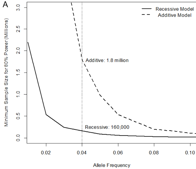
Supplemental Figure 1: Power simulation comparing additive and recessive model. Panel A shows results for a recessively acting variant with OR 2.63, equal to that of variant rs115018790 in the discovery cohort. The vertical dotted line represents the actual minor allele frequency (0.04) of rs115018790. Panel B shows results at the low end of the allele-frequency spectrum for two different ORs. Lines for recessive models are solid, and for additive, dashed.
