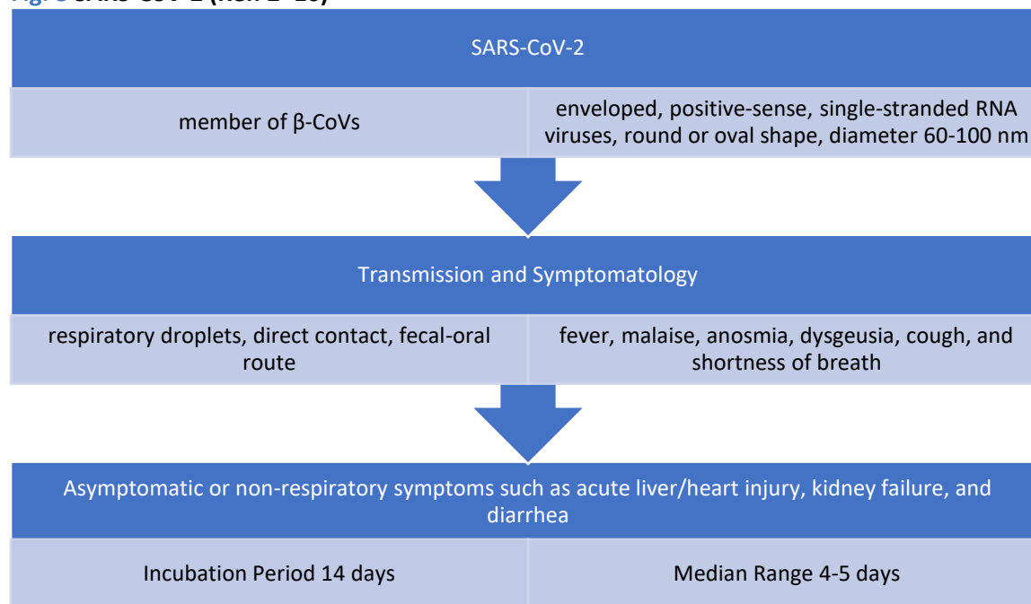
Fig. 8 SARS-CoV-2 (Ref. 2- 10)
