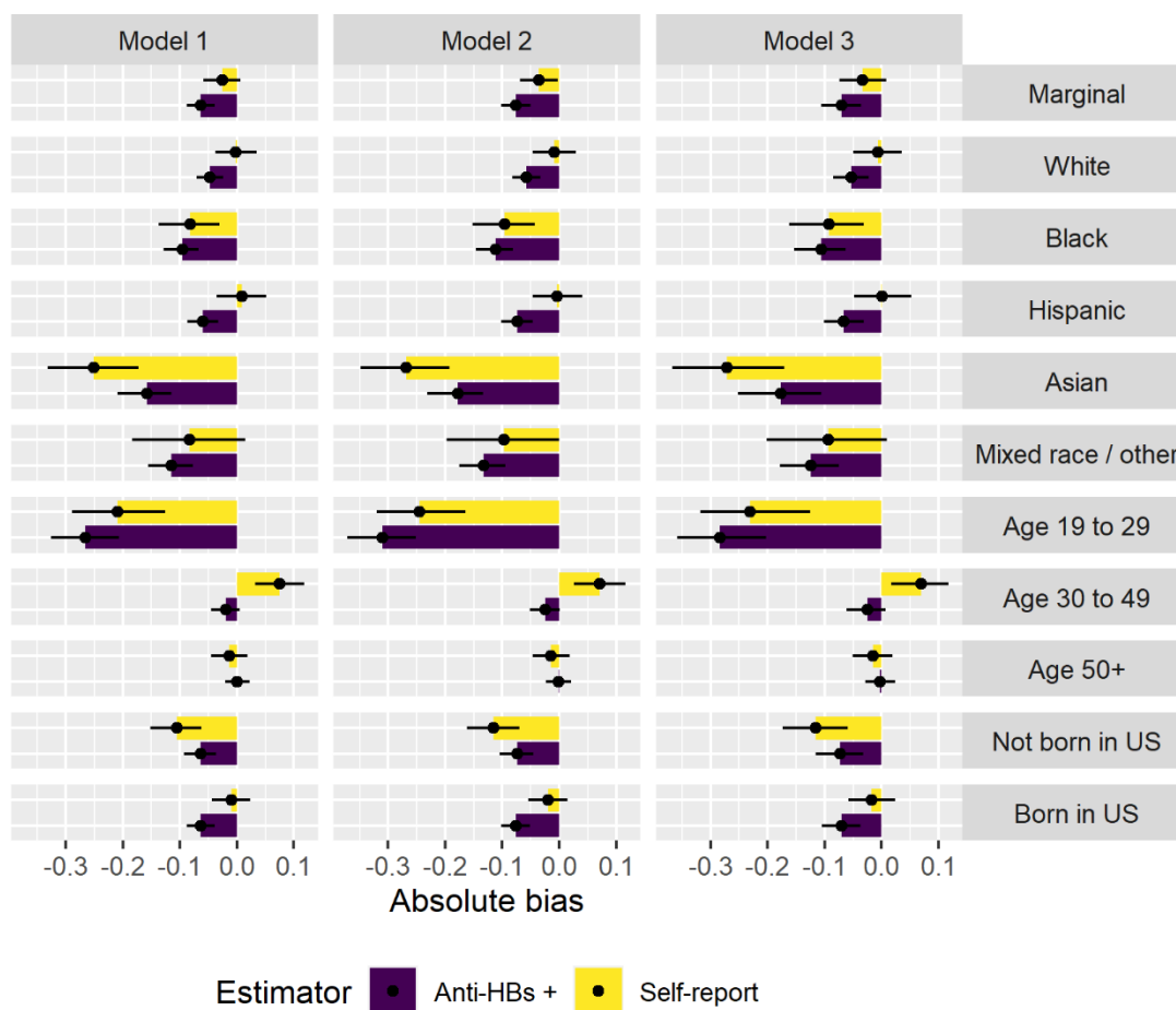
Figure 3: Absolute bias of naïve (anti-HBs or self-report) compared to bias-adjusted estimators of HBV immune prevalence by model and demographic group.
