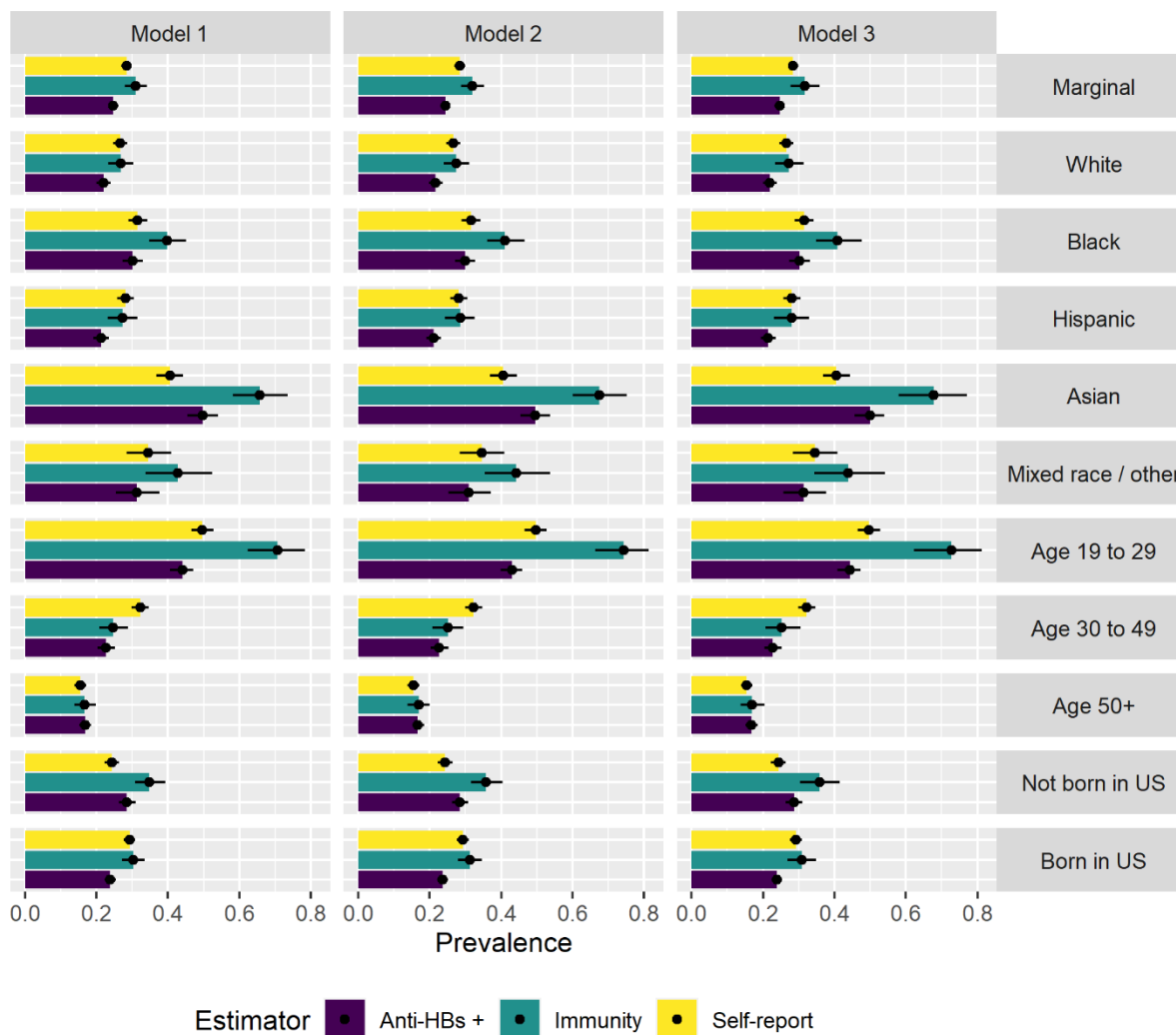
Figure 2: Estimated prevalence of immunity, anti-HBs, and self-reported vaccination by model and demographic group.
