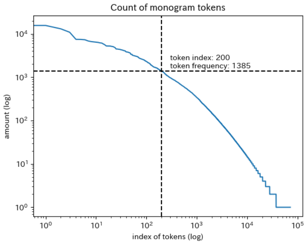
Figure 1 Count of monogram (unigram) tokens. The horizontal axis is the index of tokens by the frequency of appearance and the vertical axis is the count of appearance of the tokens.
