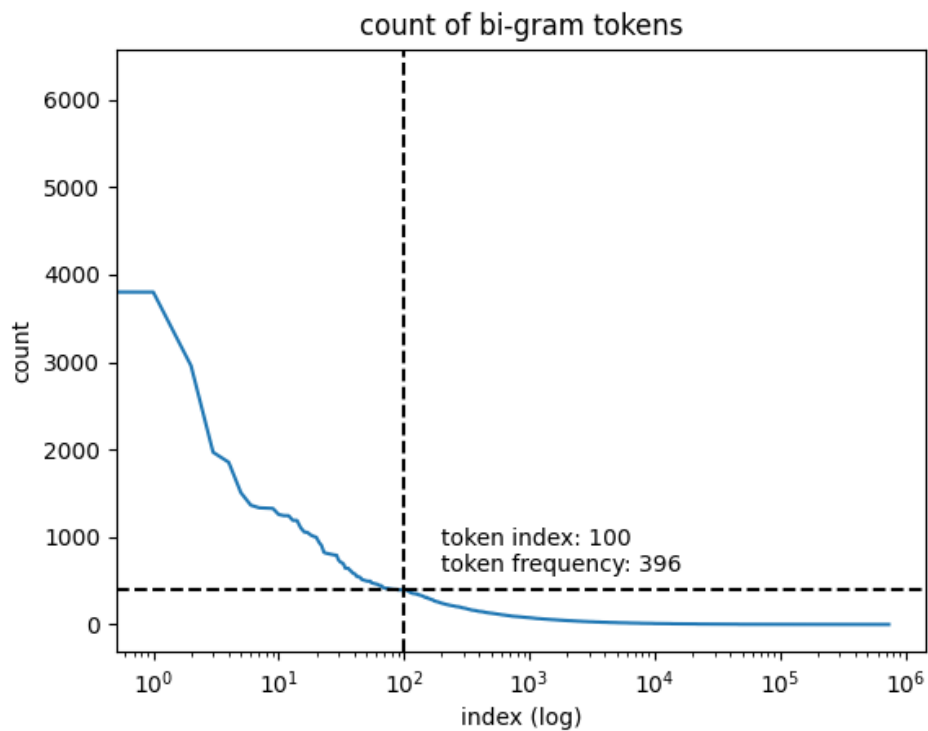
Figure 2 Count of bigram tokens. The horizontal axis is the index of tokens by the frequency of appearance and the vertical axis is the count of appearance of the tokens.
