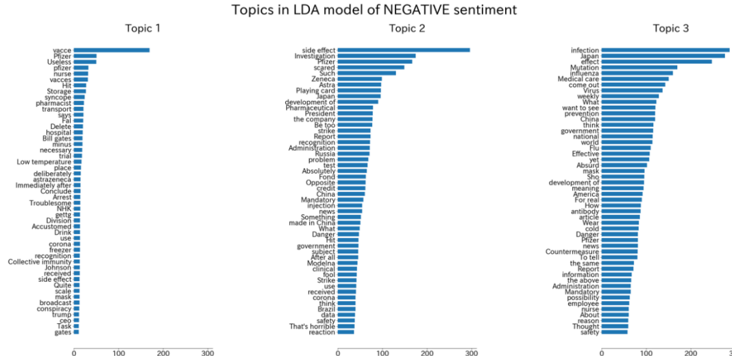
Figure 17. Top-50 words of three LDA topics for negative tweets (English version).
