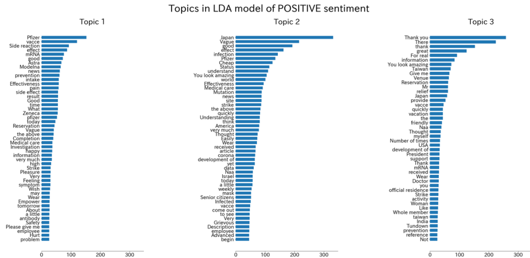
Figure 15. Top-50 words of three LDA topics for positive tweets (English version).
