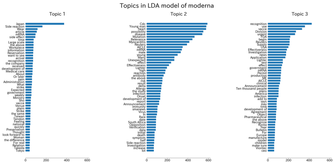
Figure 13. Top-50 words of three LDA topics for tweets related to Moderna vaccine (English version).
