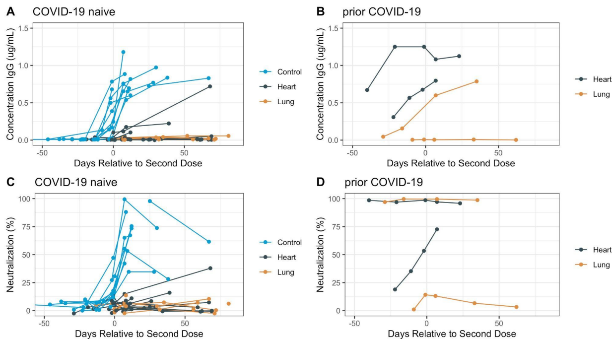
380 Figure 3: Antibody trajectories over time in individual subjects. (A-B) IgG binding to 381 SARS-CoV-2 spike protein RBD over time, as measured by IgG ELISA, in COVID-19 naive 382 subjects (A) or in subjects with prior COVID-19 infection (B) displayed by transplanted organ 383 type. Neutralization activity over time in COVID-19 naive subjects (C) or in subjects with prior 384 COVID-19 infection (D). All data points are shown.
