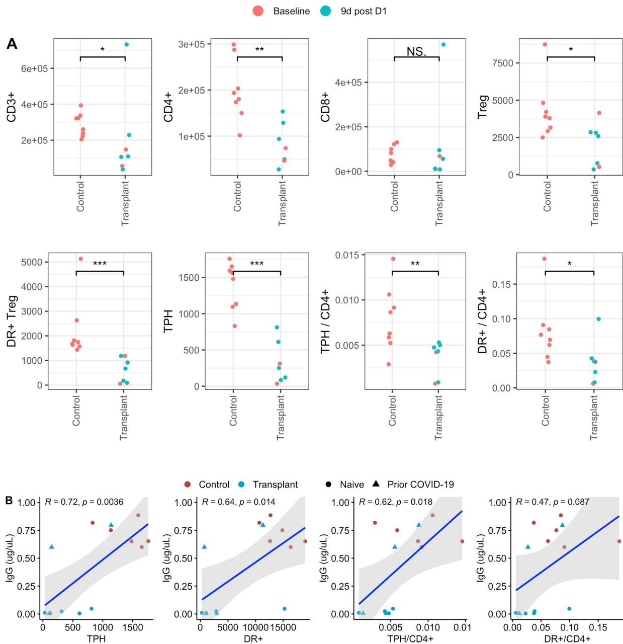
387 Figure 4: Immune cell subsets and cellular correlates of antibody response. (A) 388 Quantification by flow cytometry of peripheral blood cells in COVID-19-naive individuals. (B) 389 Correlation between antibody response at day 8 after complete vaccination and baseline levels of 390 DR+ CD4 T peripheral helper (TPH) cells; DR+ CD4 T cells; DR+ CD4 T cells as a proportion 391 of total CD4+ cells at baseline, or TPH cells as a proportion of total CD4+ cells at baseline. 392 Least squares regressions (blue lines). Gray shading, 95% confidence interval (CI). R , correlation 393 coefficient. All data points are shown. *, p < 0.05 ; **, p < 0.01 ; ***, p < 0.001 ; ****, p < 394 0.0001 .
