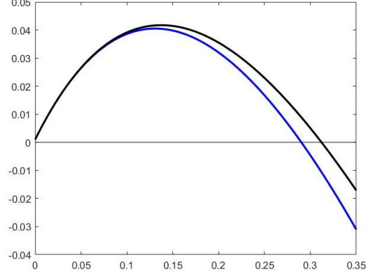
Figure 5: \tilde{i}_1 (black) for the same example as in Fig 1 and \tilde{i}_0 (blue) using the choice of \alpha and \omega stipulated in Theorem 4.1.
