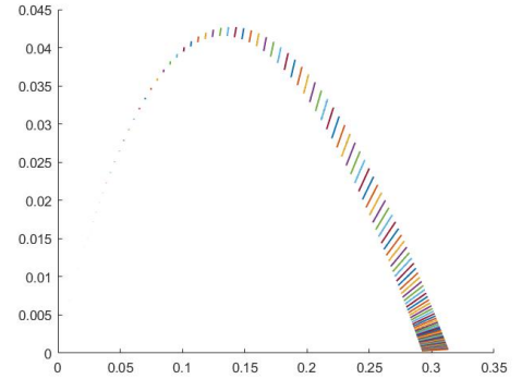
Figure 6: Line between pairs (i_0(t), r_0(t)) and (i_1(t), r_1(t)) for a grid of t -values, using the same parameters as in Fig. 1. Note that the inner and outer envelope is given by \tilde{i}_0 and \tilde{i}_1 (cf. Fig. 5).
