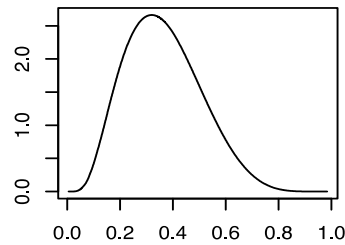
PostDens [Phi for i.spat1]
