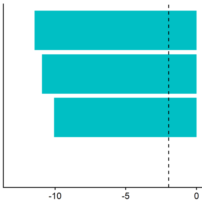
Z score of ADAMTS7 -> CAD
