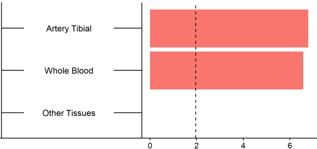
Z score of ADAMTS7 -> Pneumonia
