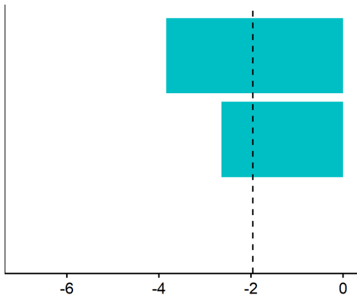
Z score of ADAMTS7 -> CAD
