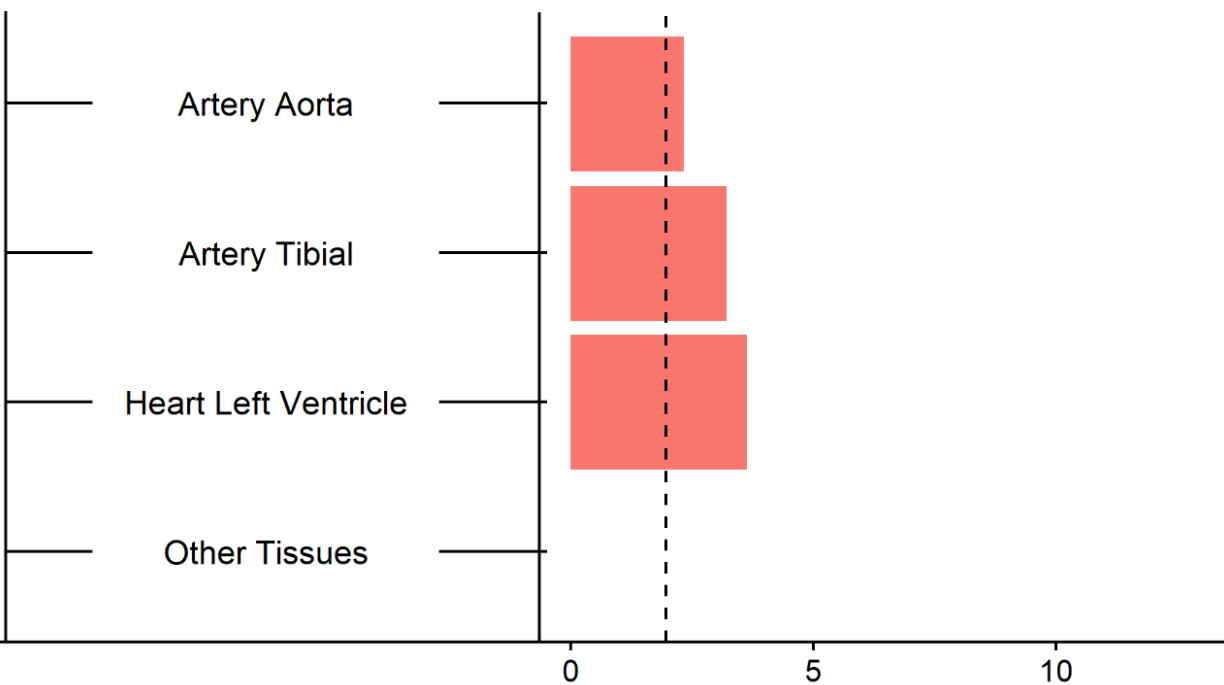
Z score of ADAMTS7 -> Pneumonia
