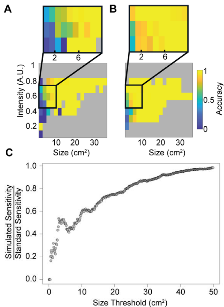
Fig. 4. Detection sensitivity as a function of lesion size and scaled intensity. Sensitivity of the deep learning classifiers for detecting lesions in the validation set is shown in the (A) simulated ULF and (B) standard HF images. Areas highlighting discrepancies between the datasets are highlighted in image insets. (C) Sensitivity of lesion detection in simulated ULF images relative to HF images. Each point represents the sensitivity ratio measured on all lesions smaller than the given size threshold. Note that sensitivity is similar between image types when averaged over all lesions but differs significantly when restricted to smaller lesions.
