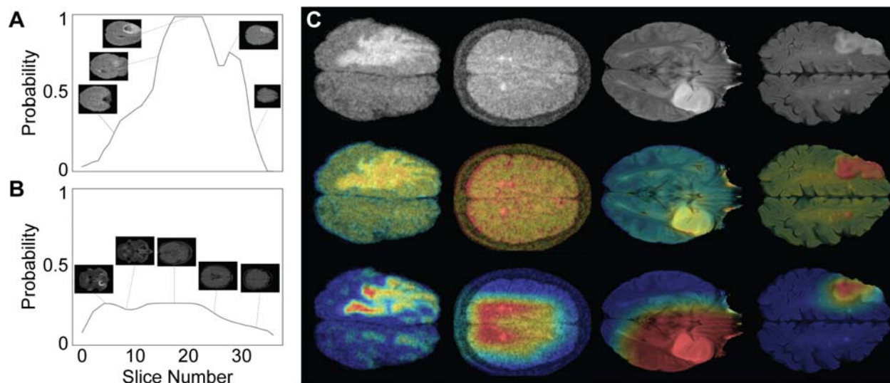
Fig. 5. Model validation and interpretability. Panel A and B provide examples of per-subject pathology detection. Convolutional filters were used to generate average lesion probability values across several adjacent axial slices. A threshold value for subject-level classification was determined empirically by maximizing per-subject classification accuracy in the training set. Sample plots are shown for a subject with HGG (A) and a control patient (B) using simulated low-field imaging. (C) Class activation mapping. Row 1: Sample images of high-grade glioma (low-field), multiple sclerosis (low-field), low-grade glioma (standard), and ischemic stroke (standard). Row 2: CAMs generated from shallow network layer for each pathology. Row 3: CAMs generated from deepest convolutional network layer for each pathology.
