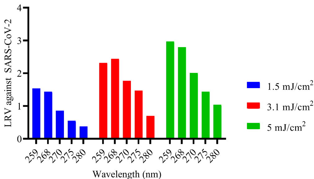
7 8 Fig 2: Effects of UVC LEDs with different peak emissions on SARS-CoV-2 (Strain USA/WA1- 9 2020) inactivation. Inactivation efficacy of wavelengths was carried out at similar UVC doses. 10 Inactivation of SARS-CoV-2 revealed wavelength sensitivity, with the 268 nm array obtaining 11 comparable performance with the 259 nm.
