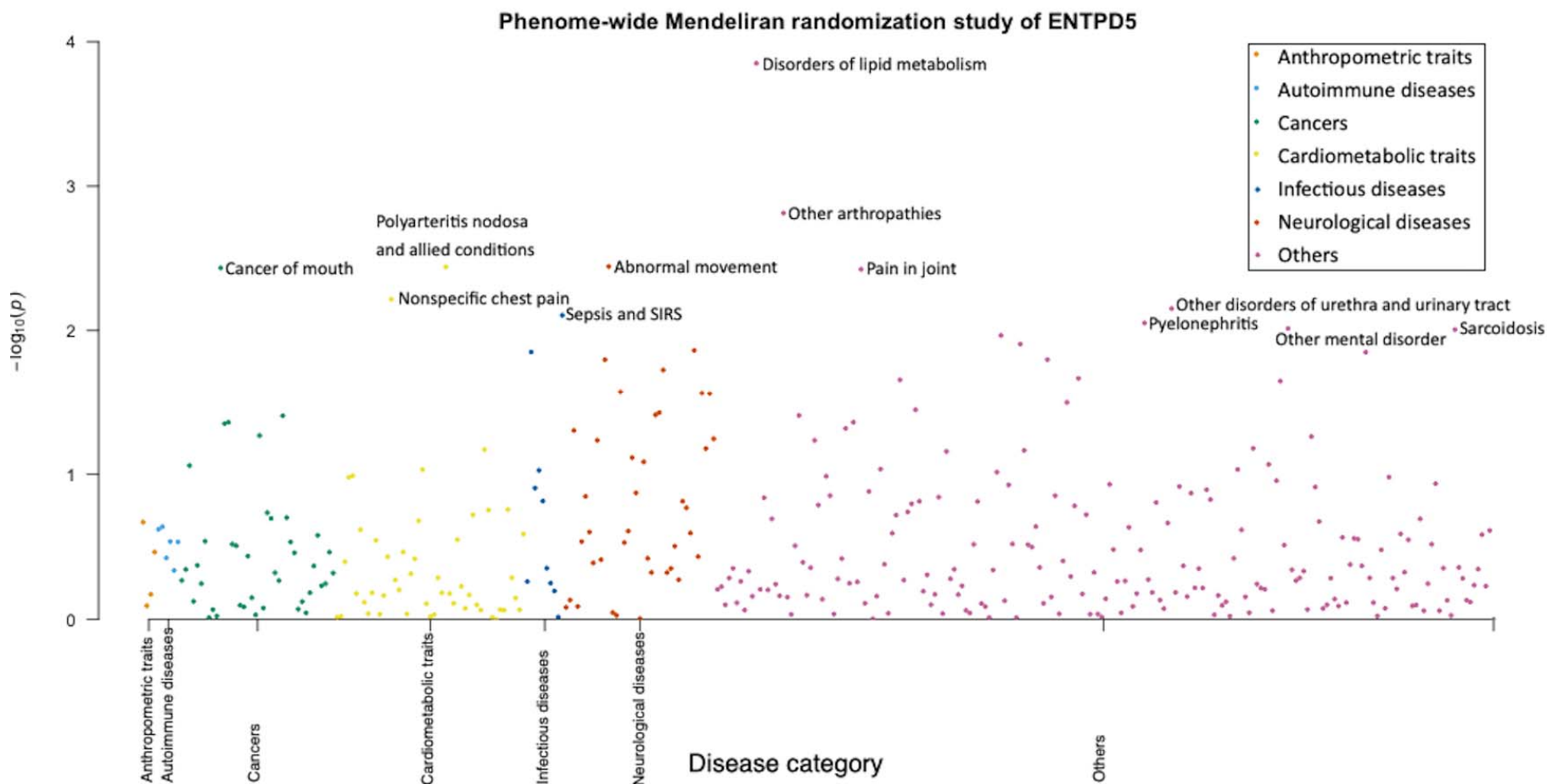
Figure 3. Manhattan plot demonstrating phenome-wide Mendelian randomization associations of protein expression level of ENTPD5 on human phenotypes. Different colors refer to different disease areas. For the 622 tested traits, none of them passed the Bonferroni-corrected threshold is 8.04 \times 10^{-5} . Therefore, ENTPD5 are less likely to be influenced by horizontal pleiotropy.
