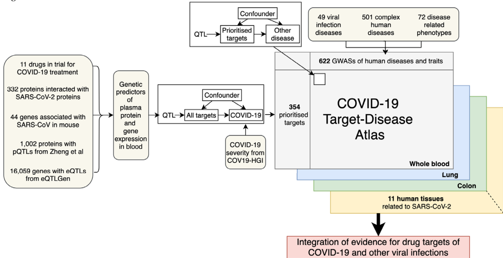
Figure 1. Study design of the multi-omics MR study to prioritise drug targets for COVID-19 severity.
