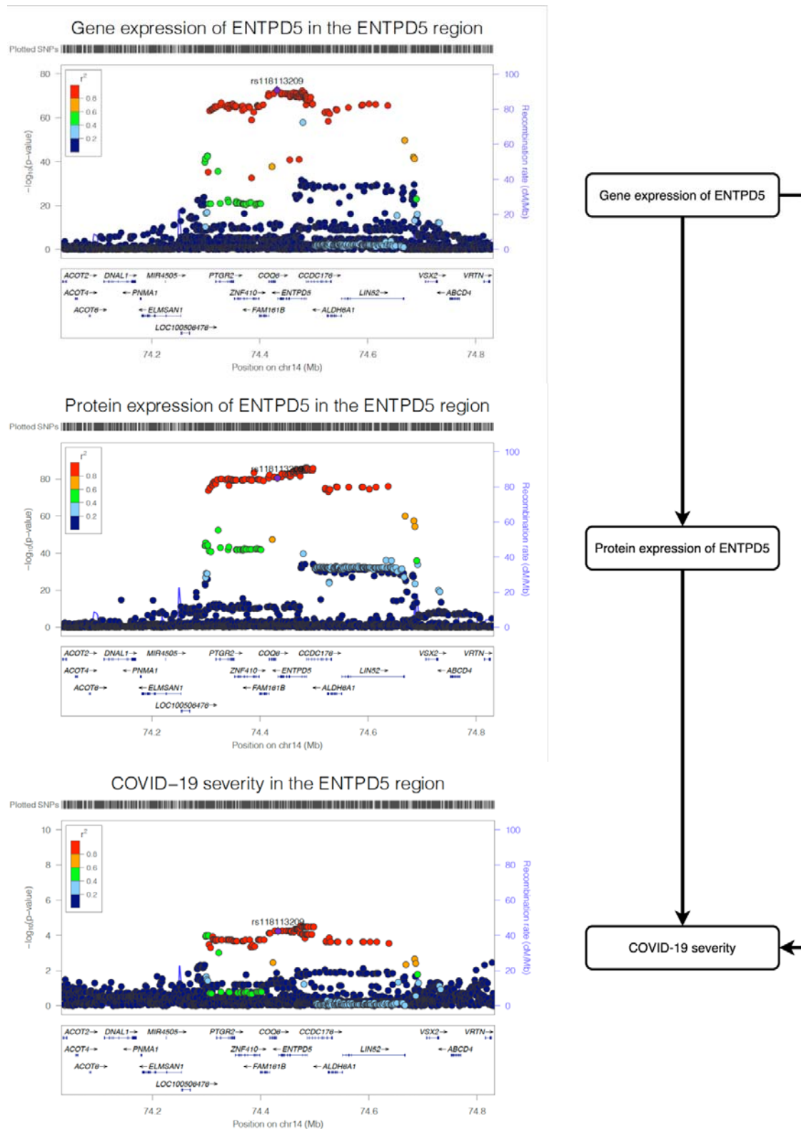
Figure 2. Regional plot of gene expression of ENTPD5 , protein expression of ENTPD5 and COVID-19 severity in the ENTPD5 region. The three regional plots refer to the genetic associations of (A), gene expression of ENTPD5 ; (B) protein expression of ENTPD5 ;
