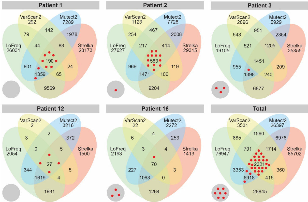
Supplementary Figure 1. No Additional Immunogenic Mutations Identified by LoFreq. Comparison of the number of neoantigens derived from single nucleotide variants (SNVs) and small insertions and deletions (indels) identified by each of four different programs (Varscan, GATK Mutect2, Strelka, and LoFreq). Red dots represent the validated immunogenic neoantigens from each patient, and the grey circle represents validated immunogenic neoantigens that were not identified by these four programs.
