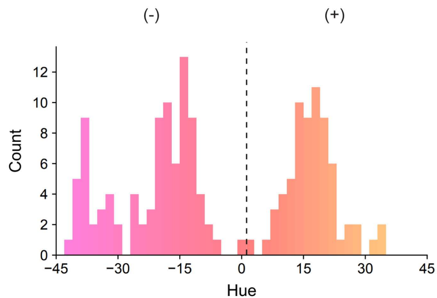
Figure 4: Colorimetric variation of LAMP reactions across different SARS-CoV-2 negative and positive saliva samples
