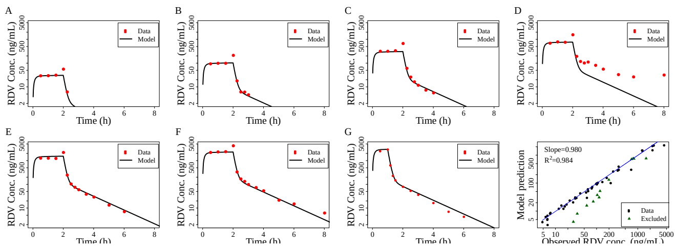
Figure S1. Median RDV plasma concentration from single dose experiments (Humeniuk et al. 2020, main text ref. 15), with different RDV dose sizes and infusion durations, compared to our pharmacokinetic model prediction (Equation (1), main text). (a) 3 mg dose for a 2 h infusion; (b) 10 mg dose for a 2 h infusion; (c) 30 mg dose for a 2 h infusion; (d) 75 mg dose for a 2 h infusion; (e) 150 mg dose for a 2 h infusion; (f) 225 mg dose for a 2 h infusion; (g) 150 mg dose for a 1 h infusion (first administration of RDV from a multi-dose study). (f) Linear regression comparing the model predictions with the data to demonstrate how well the model explains the data. Data from 75 mg dosing excluded in the fitting are marked in green.
