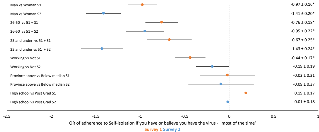
Figure 2b. Forest plot of adjusted odd ratio of adherence to self-isolation ‘Most of the time’ time’ as a function of sociodemographic characteristics among Canadian participants in two online surveys in the iCARE study in April and June 2020
