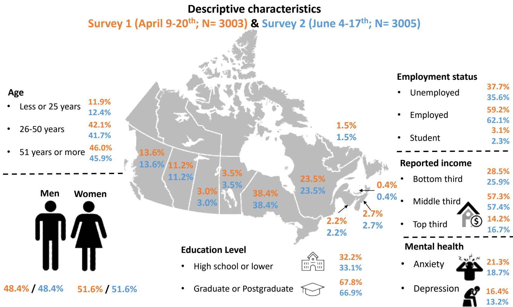
Figure 1. Selected sociodemographic characteristics of 6008 Canadian participants in two online surveys in the iCARE study in April and June 2020
