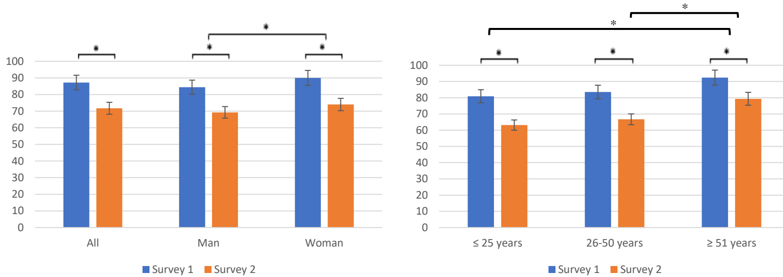
Figure 3. Proportions (95% CIs) perceiving public health measures ‘very important’ as a function of sex and age among Canadian participants to two online surveys in the iCARE study in April and June 2020
