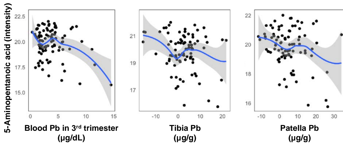
Figure 3. Scatterplots of 5-aminopentanoic acid versus Pb in 3 rd trimester blood, tibia, and patella.
