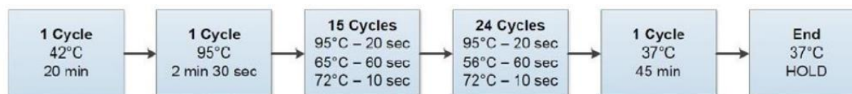
Fig 2. Thermal cycling parameters for the NxTAG® CoV Reaction Plate prior to analysis in the LUMINEX® MAGPIX® System.
