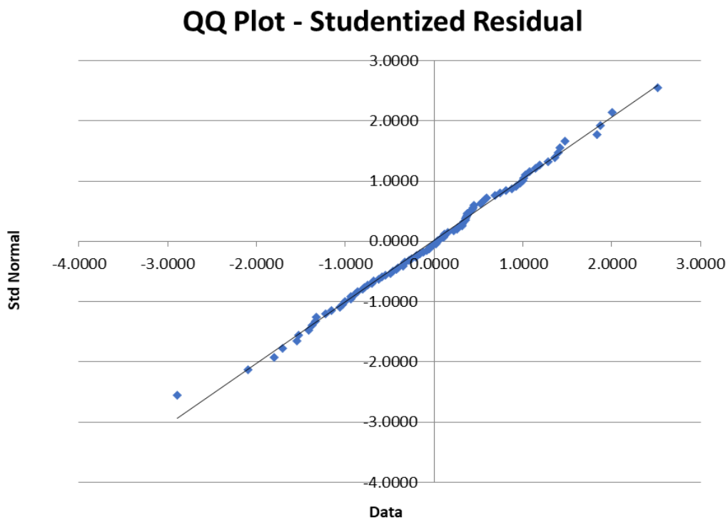
Fig. S2. QQ (Quantile-Quantile) plot of the ordered Studentized residuals vs a the corresponding quantiles of a normal distribution. Black line indicates the position of a perfectly normally distributed Studentized residuals.
