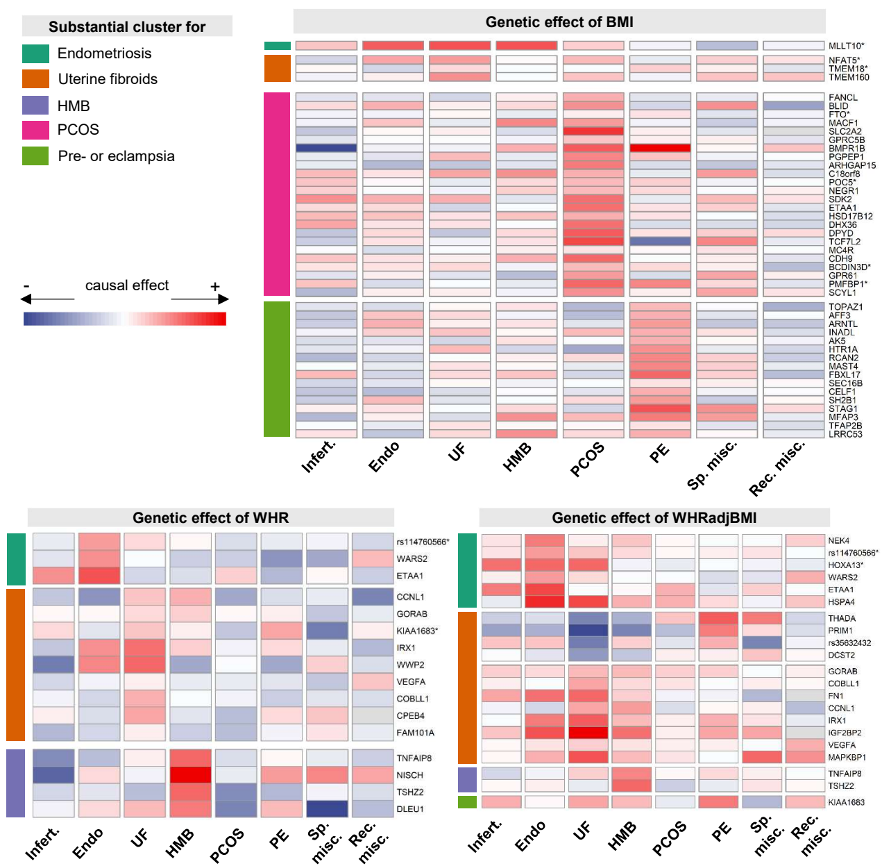
S4 Figure. Single-SNP genetic effect estimates for obesity instruments on female reproductive disorders. SNPs are annotated with their nearest gene by SNPsnap and clustered by obesity-female reproductive disorder relationship. SNPs with \geq 80\% probability of belonging to a substantial cluster (MRClust) are displayed, with an * if the SNP belongs to substantial clusters for multiple disorders. Effect size estimates are scaled to a variance of 1 within each disease.
