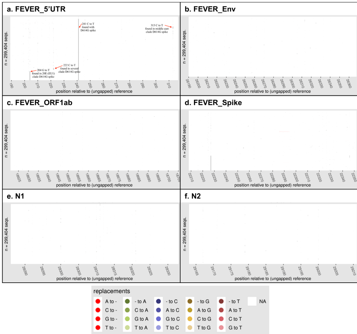
Figure S1. Visualization of SARS-CoV-2 variants in the amplified regions of FEVER and U. S. CDC RT-PCR assays. Near-complete SARS-CoV-2 sequences (n = 299,404) were assessed from GISAID.org. The amplified regions of the FEVER assays (a) FEVER_5'UTR, (b) FEVER_Env, (c) FEVER_ORF1ab, and (d) FEVER_Spike and the U.S. CDC assays (e) N1 and (f) N2 were analyzed for SARS-CoV-2 variants. In each plot, no variants (N/A) were indicated by white and genomic positions containing variants were indicated by colored dots (green, blue, yellow or red). Plots were made using the Variant Visualizer that is under development and will be available at: https://cov.lanl.gov .
