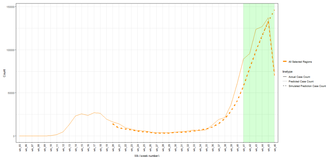
Fig 1 Validation of cases for week 46 with weeks 41 to 46 excluded from data
