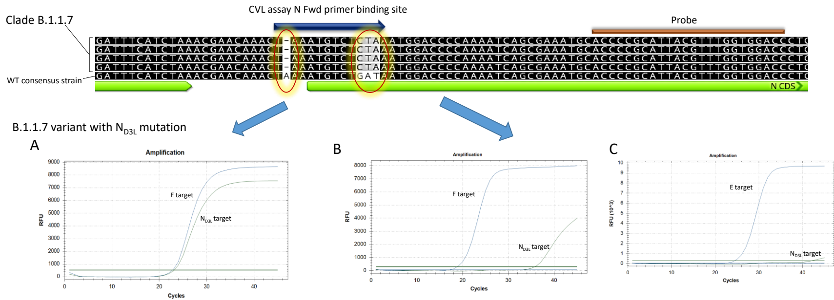
Figure 1. Design of variant B.1.1.7-specific reaction. A specific primer was designed based on the single nucleotide insertion and the codon substitution in the 5'p of the SC-2 N gene, both circled and highlighted. The specific "UK VOC" reaction was combined with an inclusive E-sarbeco reaction (Corman et al. 2020) that detects all SC-2 variants. The presence of the B.1.1.7 RNA in the assay results in two clear amplification curves (A). A sample containing a non-B.1.1.7 variant sequence results in a faint amplification, with a Cq different larger than eight between the E and the N curves (B), or a negative signal for the N reaction (C).
