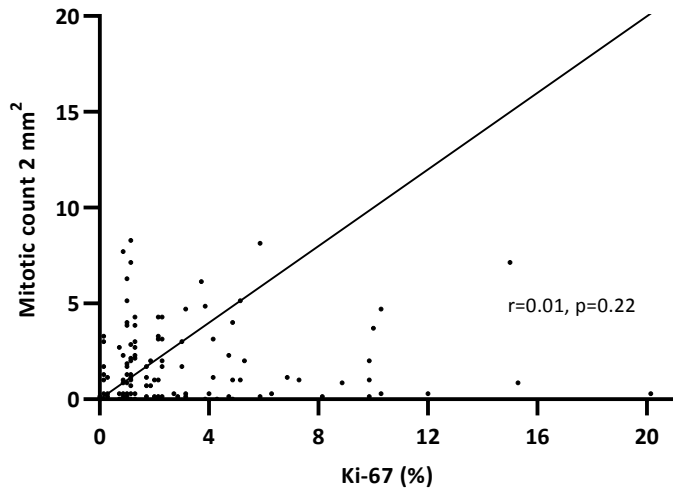
Supplementary Figure 4: correlation between Ki-67 and mitotic count, p=0.22 .
