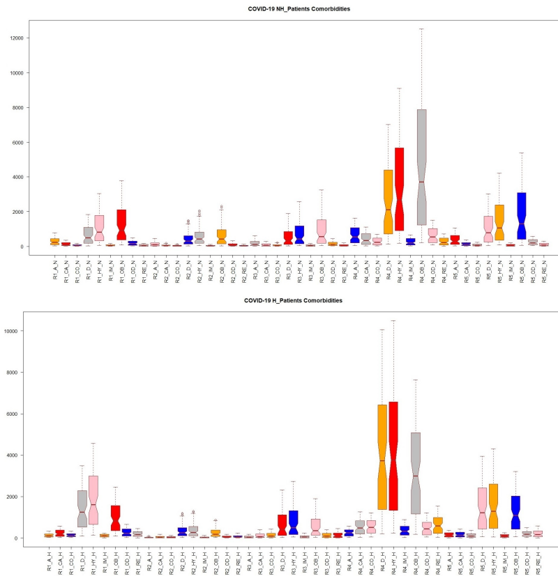
Figure 3: Box plot of the 5 Mexico's regions grouped by the 9 comorbidities, the top graph is from NH patients values and the bottom graph is form H patients.
