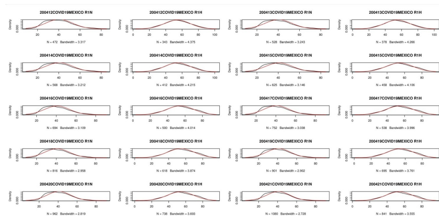
Figure 2: Age distributions plot of H and NH patients in R1 for 10 days.
