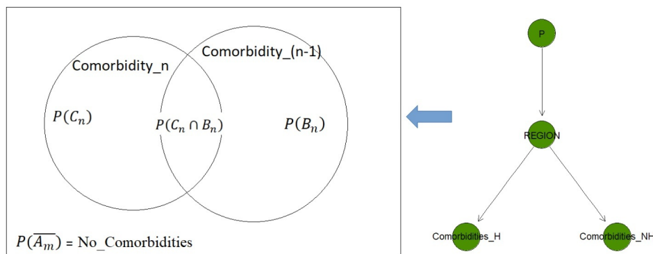
Figure 6: Bayesian Network configuration for calculate the Probability Analysis.
