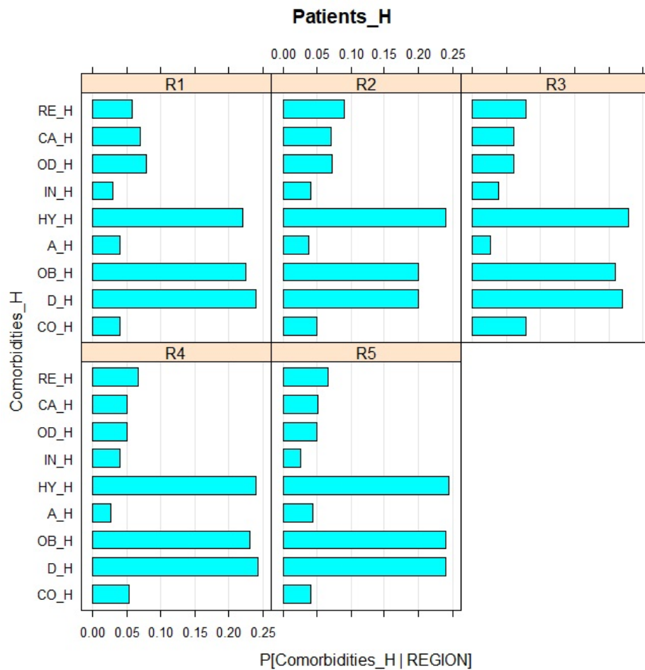
Figure 8: Network output for the Hospitalized patients and their coefficients from comorbidity probabilities for the 5 Mexico's regions in 79 days of COVID-19 registration.
