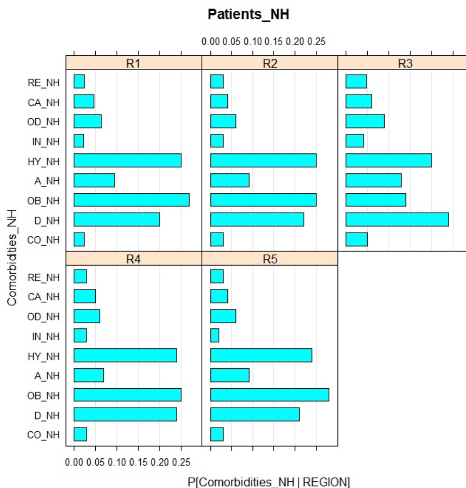
Figure 7: Network output for the Non-Hospitalized patients and their coefficients from comorbidity probabilities for the 5 Mexico's regions in 79 days of COVID-19 registration.
