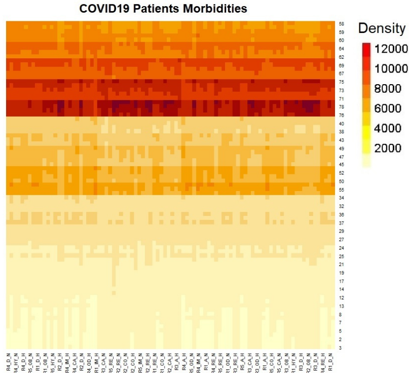
Figure 5: SuperHeat map describes the density relationship between the comorbidities, N and NH patients in the Regions of Mexico during the 79 days with the pandemic.
