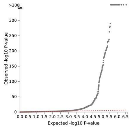
AD Genomic SEM Relaxed Model
