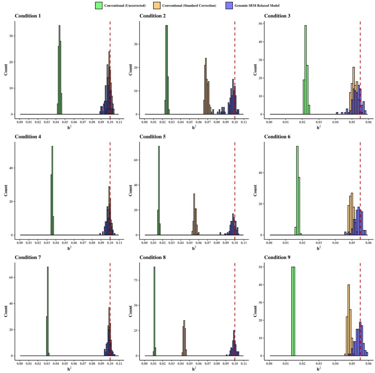
Figure S2. Simulation Results. Distribution of SNP heritability estimates ( h^2_{SNP} ) across simulation conditions.
