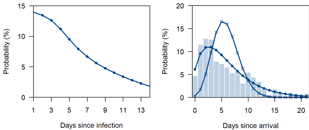
Supplementary Figure 2: Probability distribution of the duration of infection to arrival, \alpha (left) and probability distribution of time of arrival to isolation in notified imported cases with community contact; (bar) observed data, (line) model fit (dots: negative binomial, cross: Poisson)
