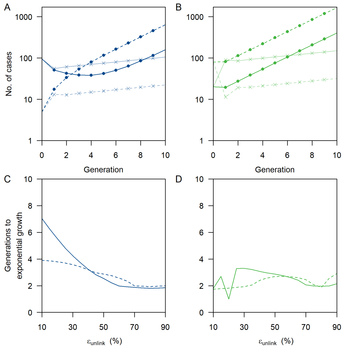
Supplementary Figure 8: Generations to exponential growth. Outbreak initiated with 5 missed imported cases (blue dashed line) and 95 notified imported cases with community contact (blue solid line), R of 1.5, \epsilon_{link} of 80%, for (A) \epsilon_{unlink} of 10% (dots) and \epsilon_{unlink} of 90% (cross); (C) varying \epsilon_{unlink} . Outbreak initiated with 80 missed imported cases (green dashed line) and 20 notified imported cases with community contact (green solid line), R of 1.5, \epsilon_{link} of 80%, for (B) \epsilon_{unlink} of 10% (dots) and \epsilon_{unlink} of 90% (cross); (D) varying \epsilon_{unlink} .
