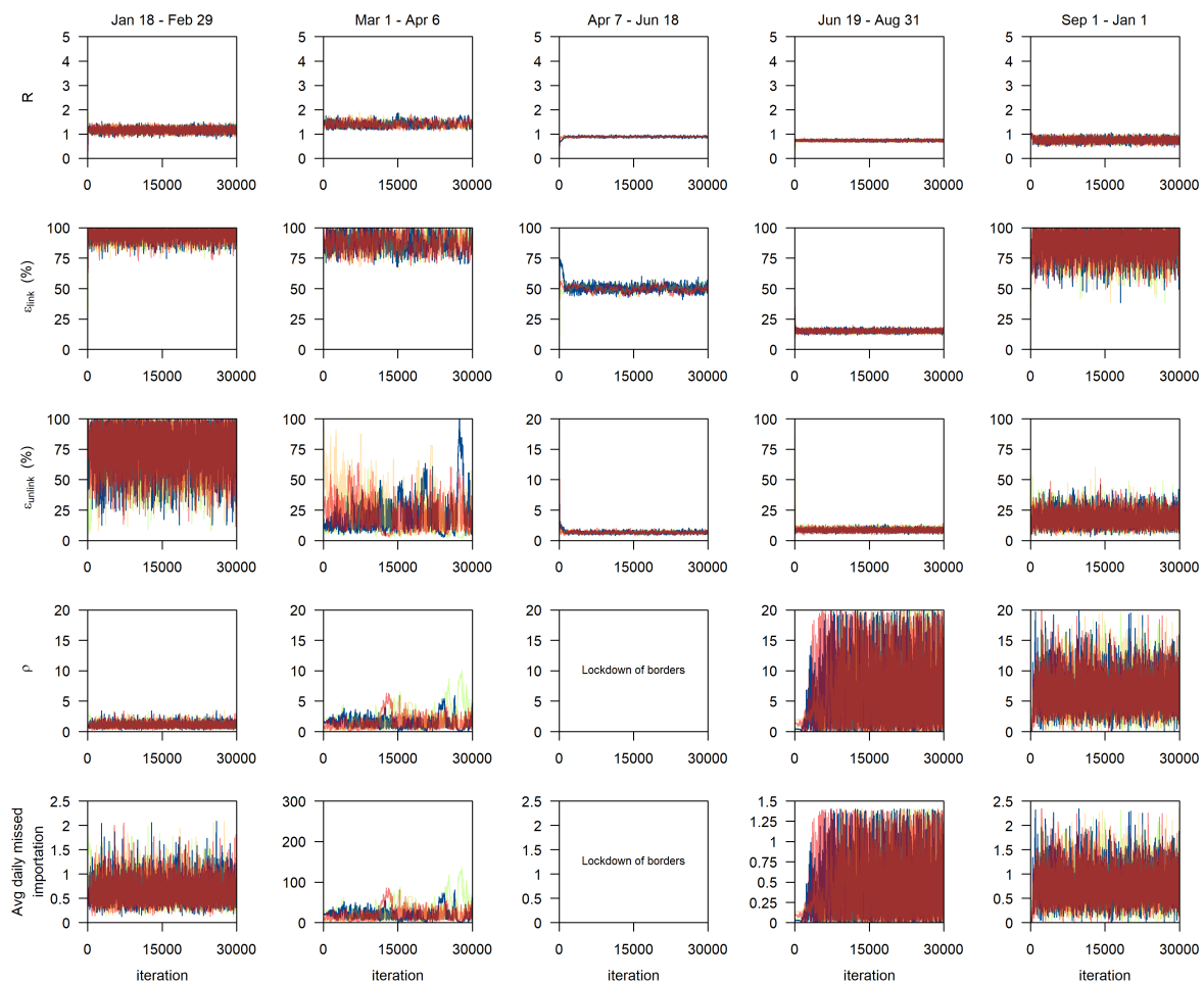
Supplementary Figure 3: Trace plot of model parameters, R (first row), \epsilon_{link} (second row), \epsilon_{unlink} (third row) and \rho (fourth row) for the first 30 000 iterations. The average daily missed
