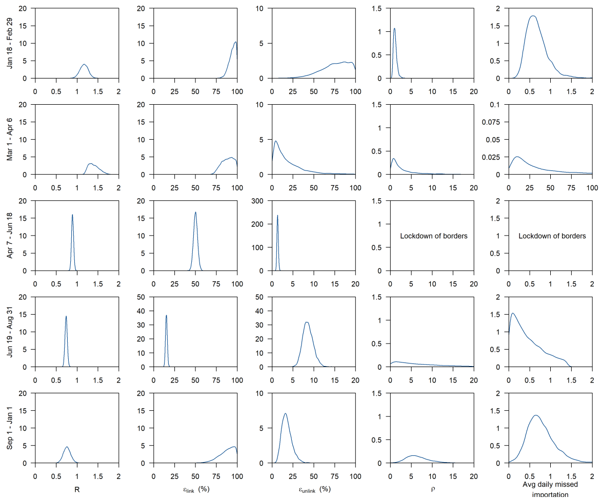
Supplementary Figure 4: Density plots of model parameters, R (first column), \epsilon_{link} (second column), \epsilon_{unlink} (third column) and \rho (fourth column). The average daily missed importation (fifth column) is the derived from \rho \bar{n}_{import} where \bar{n}_{import} is the mean daily number of notified imported cases that arrived in the time period of interest.
