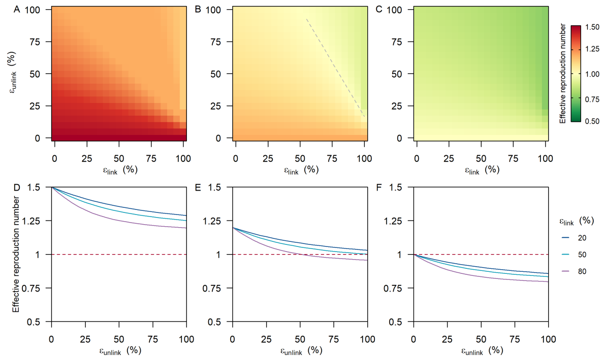
Supplementary Figure 6: Changes in effective reproduction number (i.e. R_{\text{eff}} ) for a fixed distribution of time from infection to isolation and varying \varepsilon_{\text{link}} , \varepsilon_{\text{unlink}} and potential reproduction number, R , of 1.5 (A, D), 1.2 (B, E) and 1.0 (C, F). The distribution of time from infection to isolation of notified cases follows a Weibull distribution with mean 11.0 days (SD 4.6), similar to the data observed between Jan 18 and Feb 29, 2021. (B) Grey dashed line represents effective R of 1.
