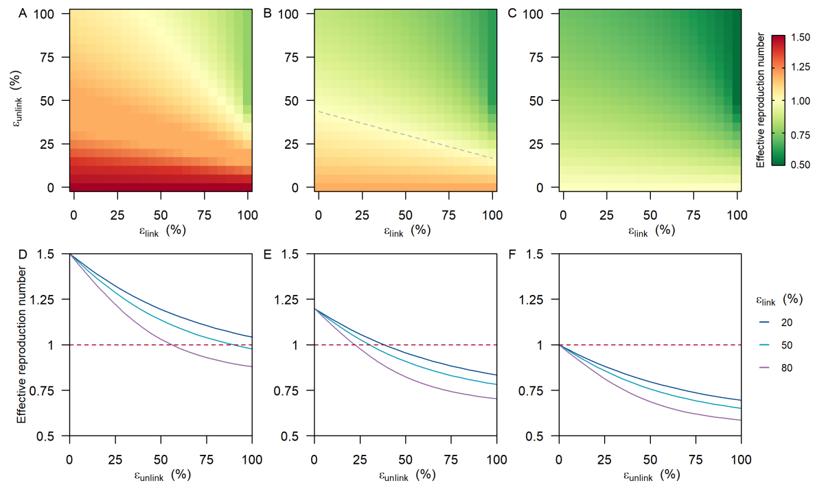
Supplementary Figure 7: Changes in effective reproduction number (i.e. R_{\text{eff}} ) for a fixed distribution of time from infection to isolation and varying \varepsilon_{\text{link}} , \varepsilon_{\text{unlink}} and potential
