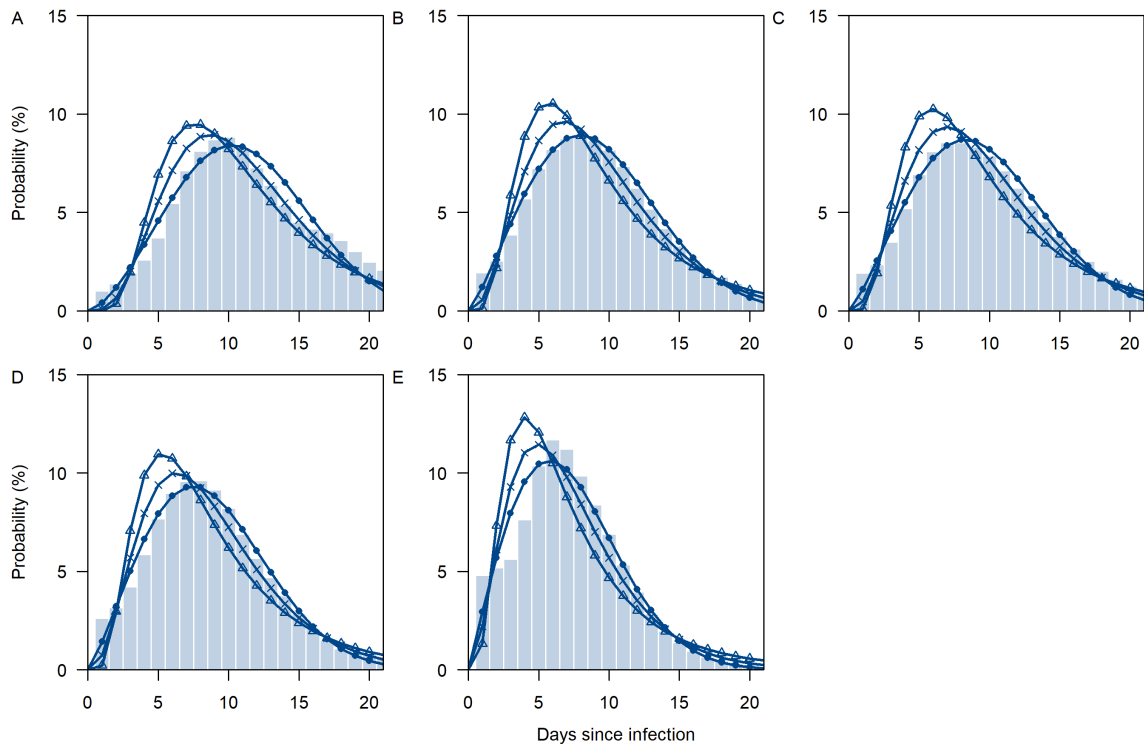
Supplementary Figure 1: Derived (bar) and model fit (dots: Weibull, cross: Gamma, triangle: Lognormal) of the marginal probability distribution of the duration of infection to isolation for community cases, \gamma . The derived distribution of \gamma was obtained by convolving the observed distribution of time from symptoms onset in notified, symptomatic community cases to isolation, and the incubation period distribution for SAR-CoV-2 infections from (A) Jan 18 to Feb 29; (B) Mar 1 to Apr 6; (C) Apr 7 to Jun 18; (D) Jun 19 to Aug 31; (E) Sep 1, 2020 to Jan 1, 2021.
