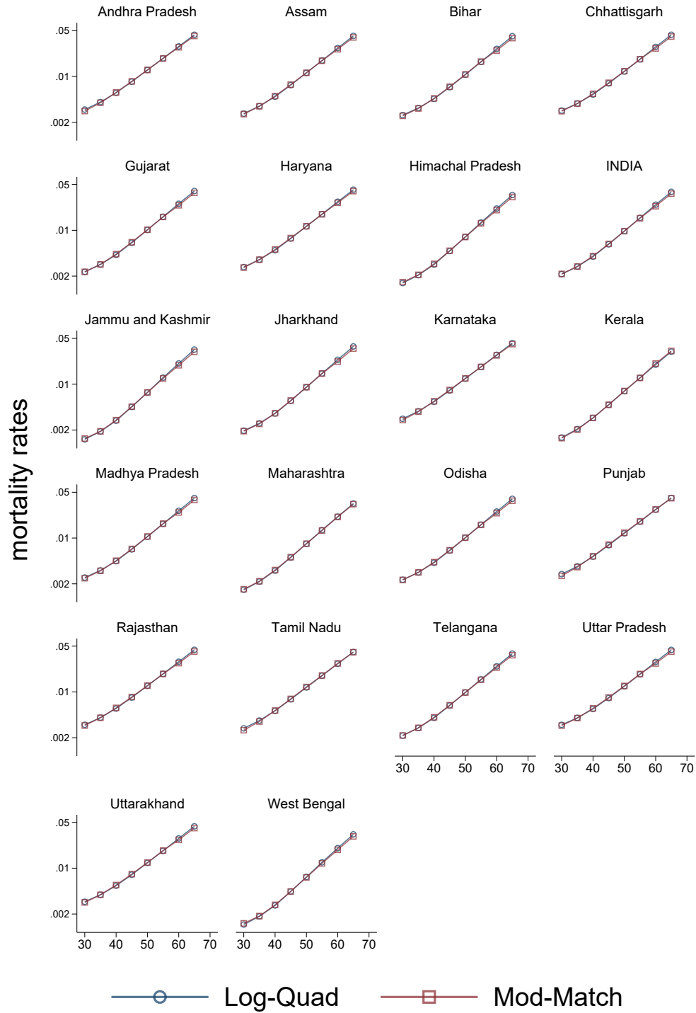
Mortality rates, Male, ages 30-70, ModMatch & LogQuad
