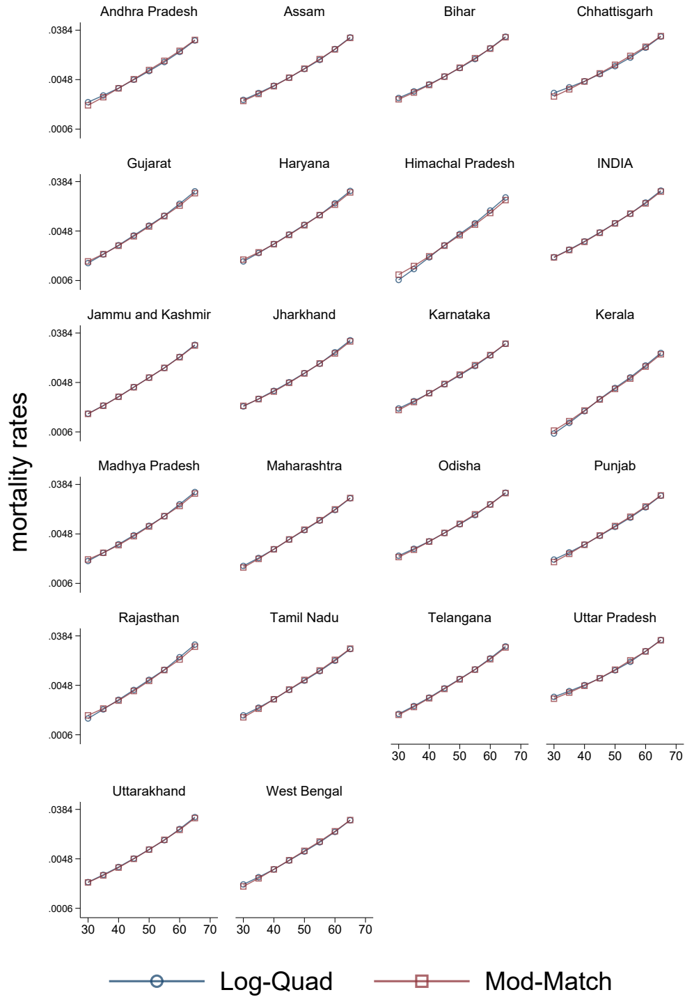
Mortality rates, Female, ages 30-70, ModMatch & LogQuad
