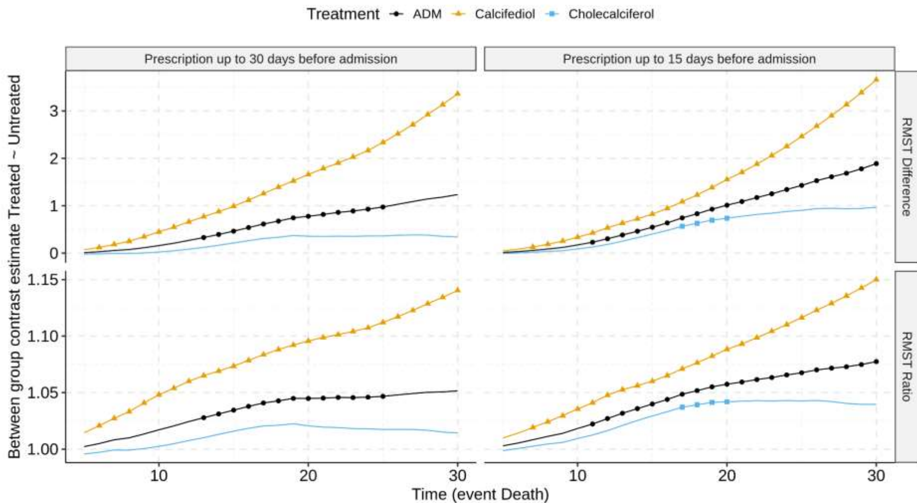
Supplementary Figure 4. RMST curves for the three treatments. RMST represents the expected survival days (on average) that subjects from the treatment group have with respect to untreated patients along time both as number of days (upper panels) or as a ratio (lower panels) for both prescriptions 15 days before admission (right panels) and 30 days (left panels). Dots (triangles, squares or circles) in the curves correspond to time points with a significant RMST, FDR-adjusted p-value < 0.05.
