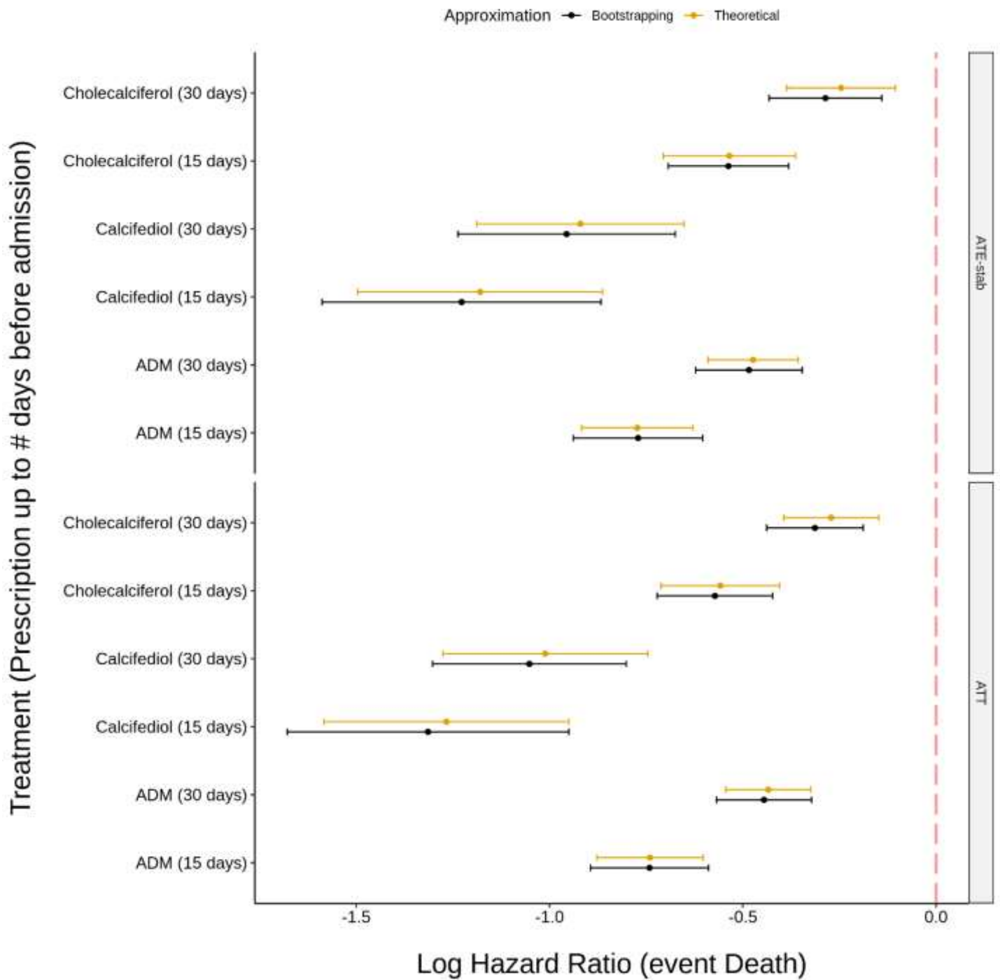
Supplementary Figure 3. Bootstrapping (n=10000 iterations) of a Cox model with the propensity weights computed by means of a Binomial General Linear Model (GLM) which regress the treatment as a function of the covariates. The bootstrapping approximates the hazard estimations of the closed form under both estimands: ATE and ATT for outcome: death.
