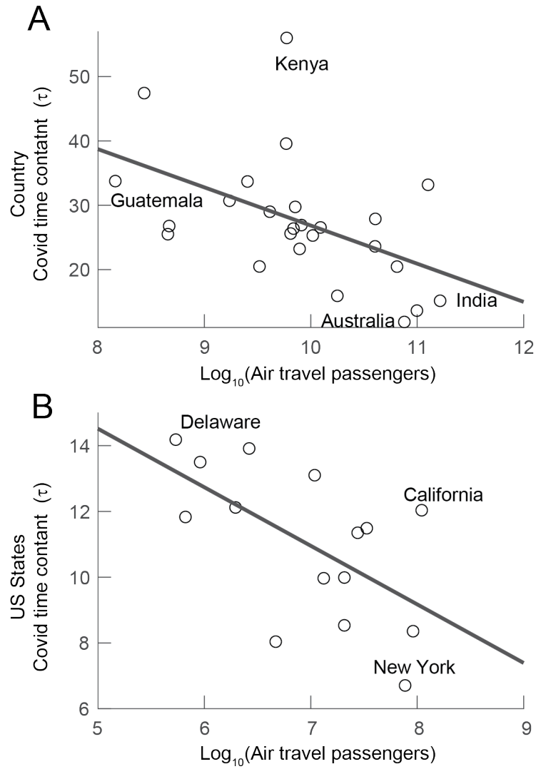
Figure S2. The time constant of the spread of the cumulative cases of COVID-19 correlate with the scale of air travel. A) The time constants obtained from fitting an exponential function to the data for the World. Only those countries that shows a better fit than the power-law were analyzed. B) The same for the amount of air travel in US states.
