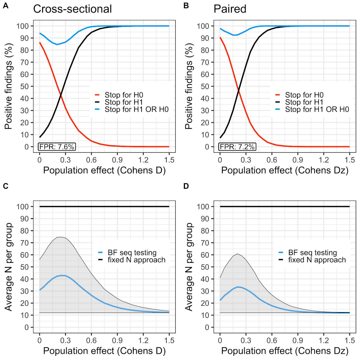
Figure S9. Settings for the simulation: H1 is a one sided cauchy(0,0.707), ( N_{start} = 12 , N_{max} = 100 , BF threshold = 4). A and B) The black curve shows the proportion of studies that showed support for H1 ( BF > 4 ) during data collection, at a range of population effects (starting at no effect, D = 0 ). The red curve is the proportion of studies showing support for H0 ( BF < 1/4 ). The blue curve is the sum of the red and black curves. C and D) shows the average number of subjects needed to reach a stopping decision at different population effects. The flat black line represents N_{max} (100 subjects/group). BF sequential testing is the blue line with shaded area denoting \pm 1 SD.
