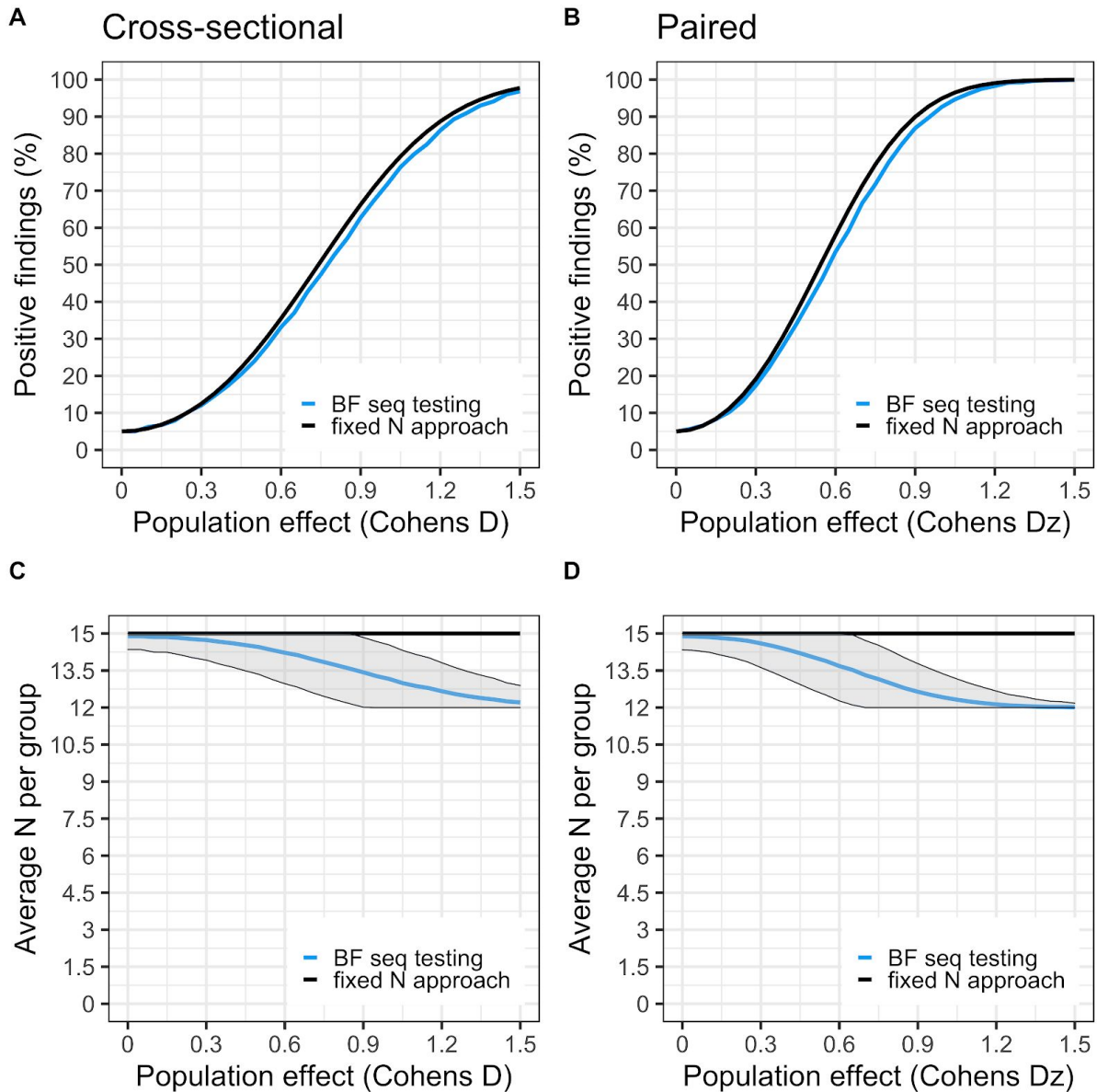
Figure S2. Settings for the simulation: H1 is a two-sided cauchy(0,0.707), ( N_{start} = 12 , N_{max} = 15 , BF threshold = 2.4 and 2.5 for cross-sectional and paired respectively). Panel A and B shows true positive (or “power”) curves for BF sequential testing (blue) and a fixed N approach (black). The curves denote the rate of true positive findings at different population effects. For the fixed N approach, only one test is performed at N=15 per group. For the sequential testing, 8 subjects/group are first collected, then BF is checked after each added comparison pair until 15 subjects/group is reached, using a stopping threshold of 4. Panel C and D shows the average number of subjects needed to reach a stopping decision at different population effects. Fixed N is the black line (fixed at N = 15 /group); BF sequential testing is the blue line with shaded area denoting \pm 1 SD.
