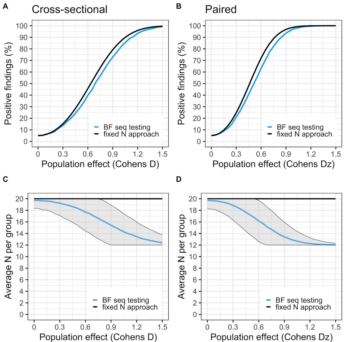
Figure S3. Settings for the simulation: H1 is a two-sided cauchy(0,0.707), ( N_{start} = 12 , N_{max} = 20 , BF threshold = 3.1 and 3.3 for cross-sectional and paired respectively). Panel A and B shows true positive (or “power”) curves for BF sequential testing (blue) and a fixed N approach (black). The curves denote the rate of true positive findings at different population effects. For the fixed N approach, only one test is performed at N=20 per group. For the sequential testing, 12 subjects/group are first collected, then BF is checked after each added comparison pair until 20 subjects/group is reached, using a stopping threshold of 4. Panel C and D shows the average number of subjects needed to reach a stopping decision at different population effects. Fixed N is the black line (fixed at N = 20 /group); BF sequential testing is the blue line with shaded area denoting \pm 1 SD.
