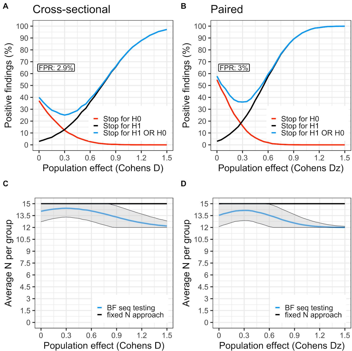
Figure S6. Settings for the simulation: H1 is a one sided cauchy(0,0.707), ( N_{start} = 12 , N_{max} = 15 , BF threshold = 4). A and B) The black curve shows the proportion of studies that showed support for H1 ( BF > 4 ) during data collection, at a range of population effects (starting at no effect, D = 0 ). The red curve is the proportion of studies showing support for H0 ( BF < 1/4 ). The blue curve is the sum of the red and black curves. C and D) shows the average number of subjects needed to reach a stopping decision at different population effects. The flat black line represents N_{max} (15 subjects/group). BF sequential testing is the blue line with shaded area denoting \pm 1 SD.
