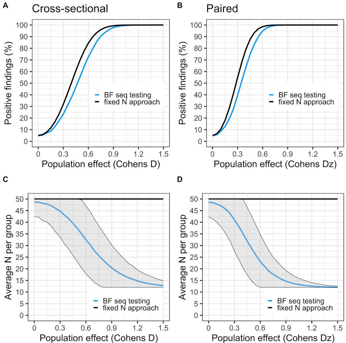
Figure S4. Settings for the simulation: H1 is a two-sided cauchy(0,0.707), ( N_{start} = 12 , N_{max} = 50 , BF threshold = 5.2 and 5.4 for cross-sectional and paired respectively). Panel A and B shows true positive (or “power”) curves for BF sequential testing (blue) and a fixed N approach (black). The curves denote the rate of true positive findings at different population effects. For the fixed N approach, only one test is performed at N=50 per group. For the sequential testing, 12 subjects/group are first collected, then BF is checked after each added comparison pair until 50 subjects/group is reached, using a stopping threshold of 4. Panel C and D shows the average number of subjects needed to reach a stopping decision at different population effects. Fixed N is the black line (fixed at N = 50 /group); BF sequential testing is the blue line with shaded area denoting \pm 1 SD.
