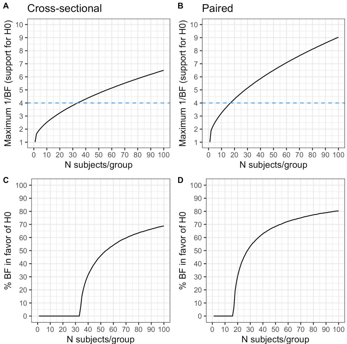
Figure S11. Maximum possible support ( 1/BF ) in favor of H_0 compared to H_1 when using a two-tailed BF t-test. A-D) When using the settings described in the main article ( H_1 is specified as a Cauchy(0,0.707) , N_{start} = 12 , threshold = 4) but a two-tailed test instead of a one-tailed test, it is not possible to obtain evidence in favor of H_0 at smaller N . E.g., in a cross-sectional design, at least 34 subjects/group are needed before the BF can reach a threshold of 1/4 . C-D) Percentage of BF showing support ( 1/BF > 4 ) for H_0 at different N . E.g., at 50 subjects/group, only 45% of BF will show support in favor of H_0 , when H_0 is true. Hence, in order to stop for H_0 when using commonly seen sample sizes in PET studies, we recommend to use a one-tailed BF t-test instead. This means that the researchers must make a prediction of the direction of the effect before initiating the study.
