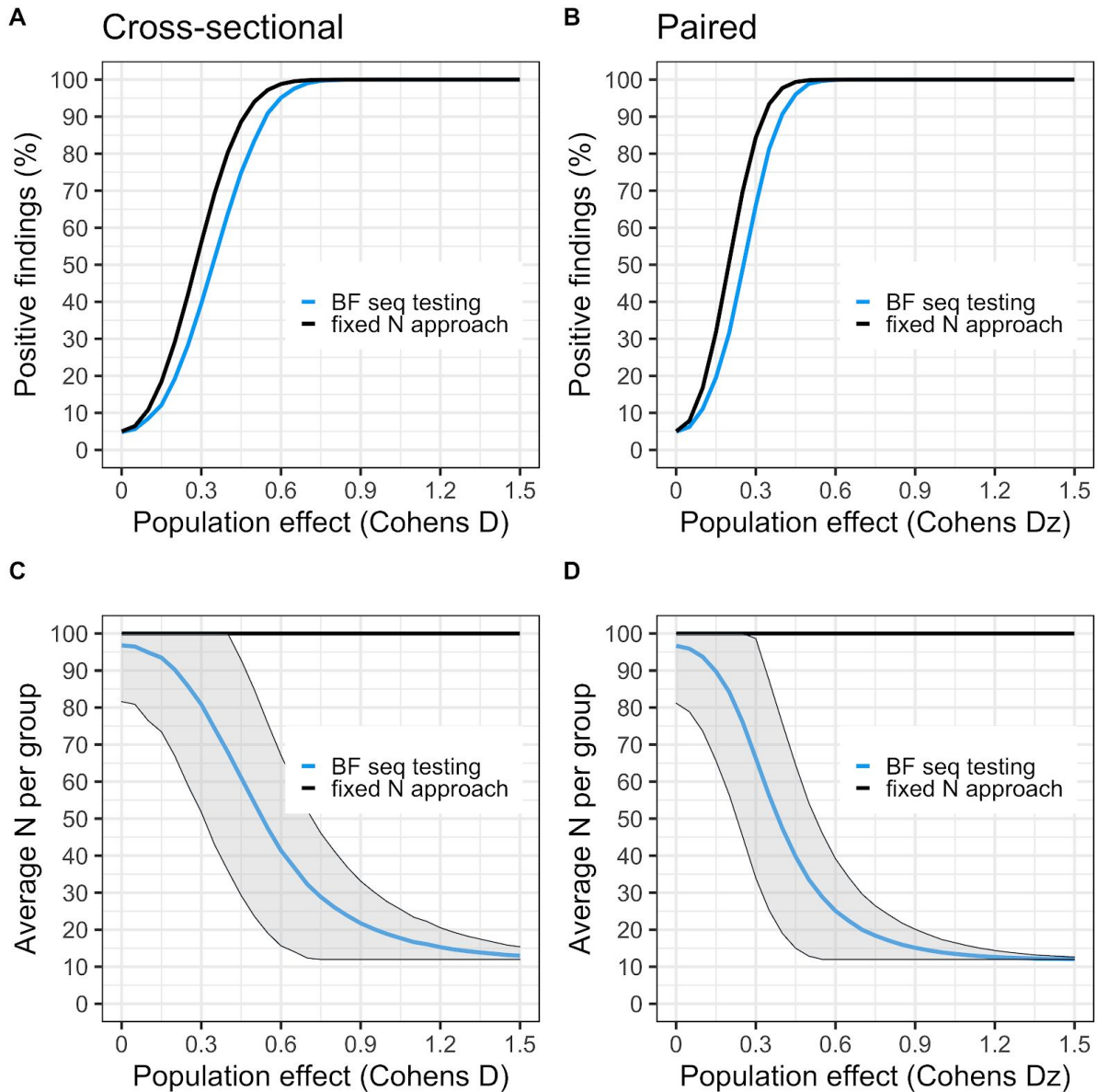
Figure S5. Settings for the simulation: H1 is a two-sided cauchy(0,0.707), ( N_{start} = 12 , N_{max} = 100 , BF threshold = 6.6 and 6.7 for cross-sectional and paired respectively). Panel A and B shows true positive (or “power”) curves for BF sequential testing (blue) and fixed N approach (black). The curves denote the rate of true positive findings at different population effects. For the fixed N approach, only one test is performed at N=100 per group. For the sequential testing, 12 subjects/group are first collected, then BF is checked after each added comparison pair until 100 subjects/group is reached, using a stopping threshold of 4. Panel C and D shows the average number of subjects needed to reach a stopping decision at different population effects. Fixed N is the black line (fixed at N = 100 /group); BF sequential testing is the blue line with shaded area denoting \pm 1 SD.
