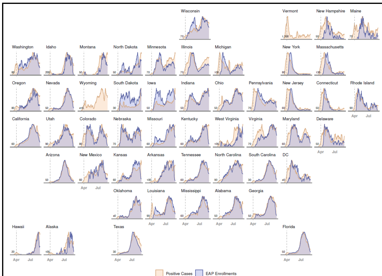
284 Figure 5. Daily rates of COVID-19-confirmed infections and patient enrollment in 285 the US Expanded Access Program (EAP). Chronological line charts represent the daily 286 number of state-wide COVID-19-confirmed infections and EAP patient enrollment 287 sequentially arranged in a geofaceted depiction of the US. Daily rates are presented as 288 a moving average across seven days, scaled between 0 (least cases/enrollments) and 1 289 (most cases/enrollments) for any day in each state. Vertical, dashed grey lines represent 290 the start date of the EAP (April 3rd, 2020). Values in the lower left corner of each panel 291 indicate the scaling factor between the two plots (cases/enrollments), which approximates 292 the number of COVID-19 cases that contributed to one enrollment in the EAP. EAP 293 enrollment data are not presented for Vermont or Wyoming because total enrollments 294 were not greater than 10 patients.
