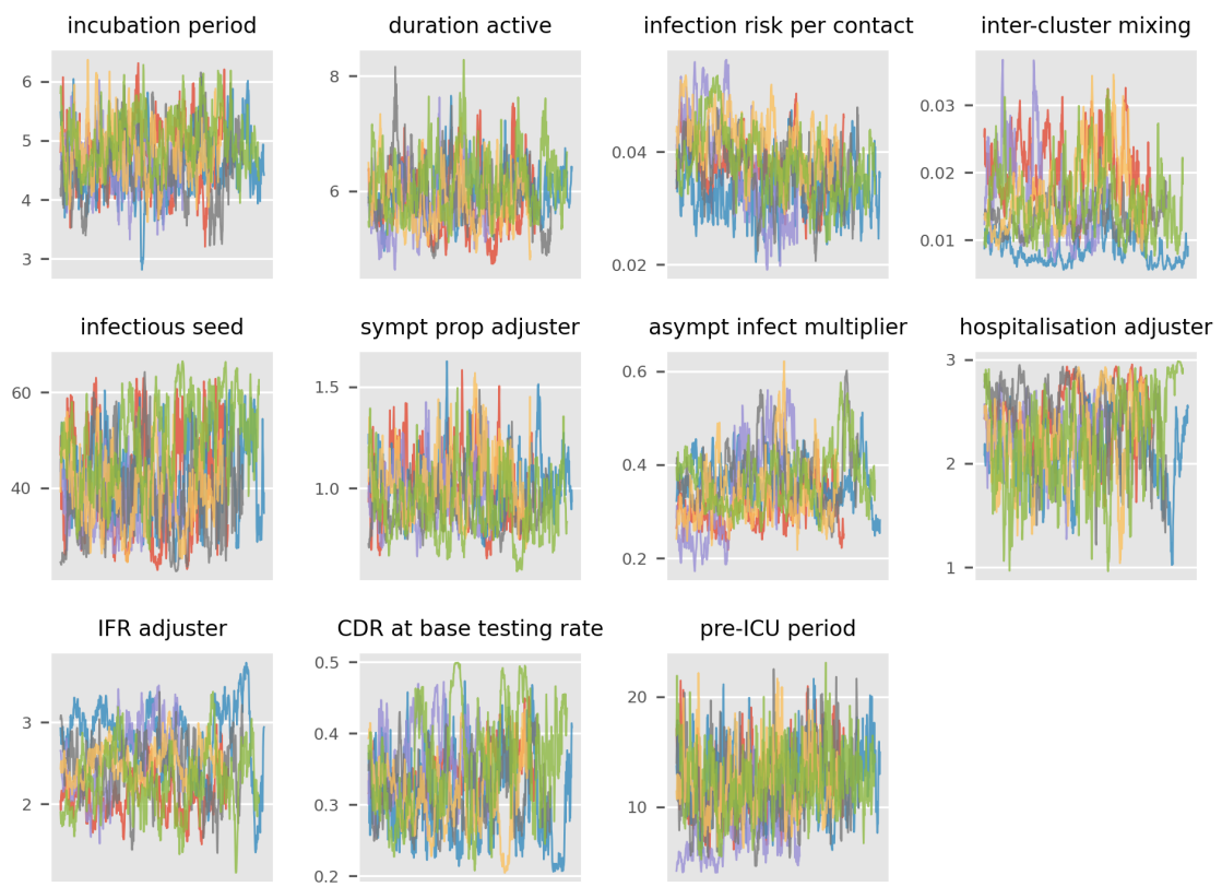
Figure 14 – Parameter progression traces for epidemiological parameters.
