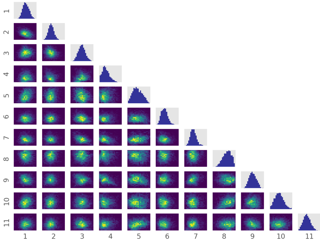
Figure 11 – Correlation matrix for other state-wide epidemiological parameters. Parameters are: 1, incubation period; 2, duration active; 3, infection risk per contact; 4, inter-cluster mixing; 5, infectious seed; 6, sympt prop adjuster; 7, asympt infect multiplier; 8, hospitalisation adjuster; 9, IFR adjuster; 10, CDR at base testing rate; 11, pre-ICU period.
