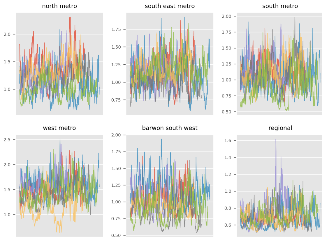
Figure 15 – Parameter progression traces for cluster contact rate modifier parameters.
