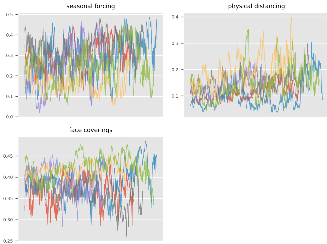
Figure 13 – Parameter progression traces for key estimation parameters.
