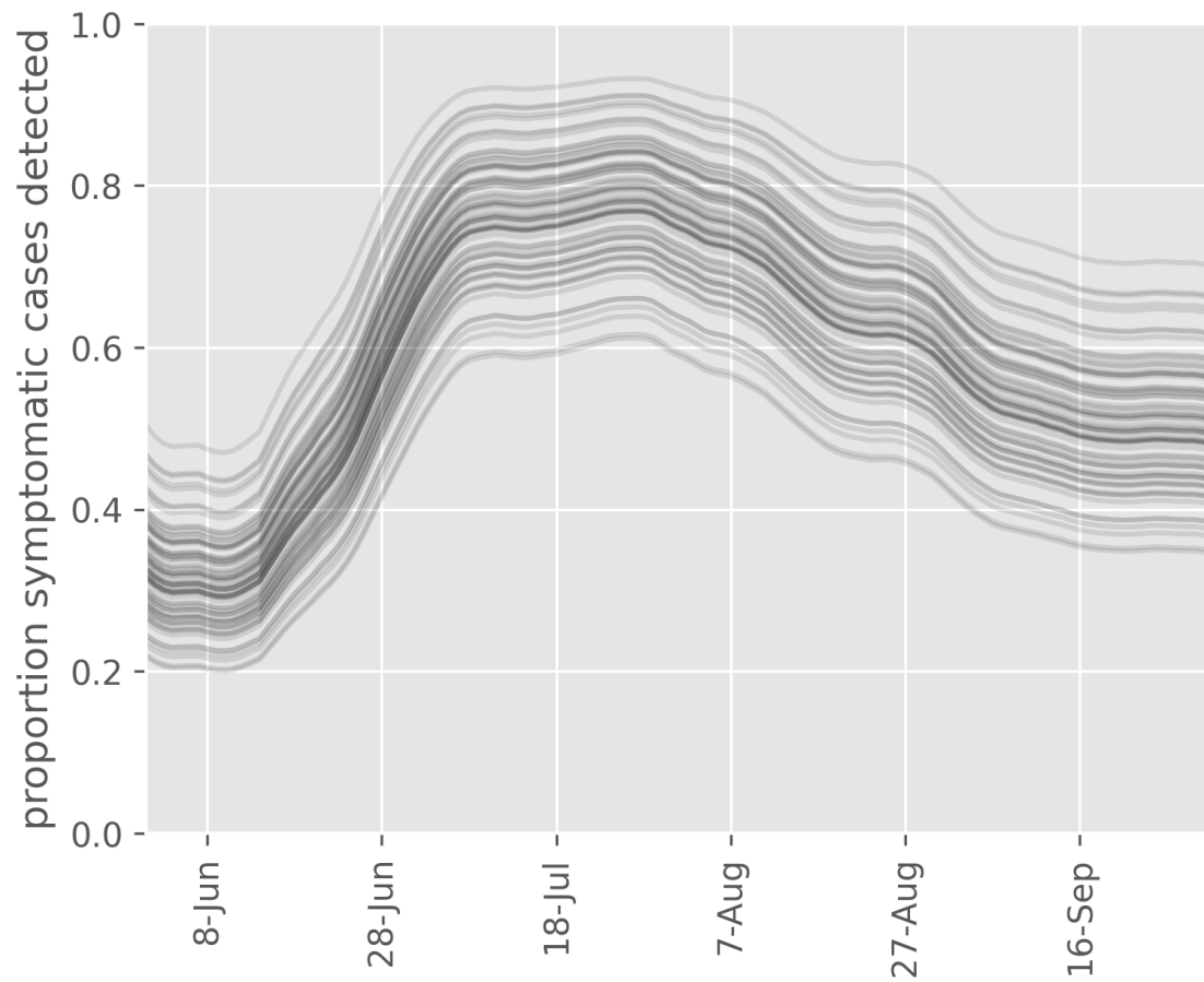
Figure 4 – Example case detection rate curves. 70 parameters for the case detection rate at a given daily per capita testing rate were sampled at random from accepted values to produce this graph.
