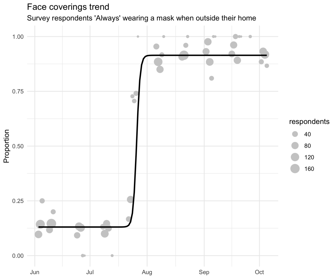
Figure 6 – Face coverings micro-distancing function for metropolitan Melbourne clusters with data used for fitting.
