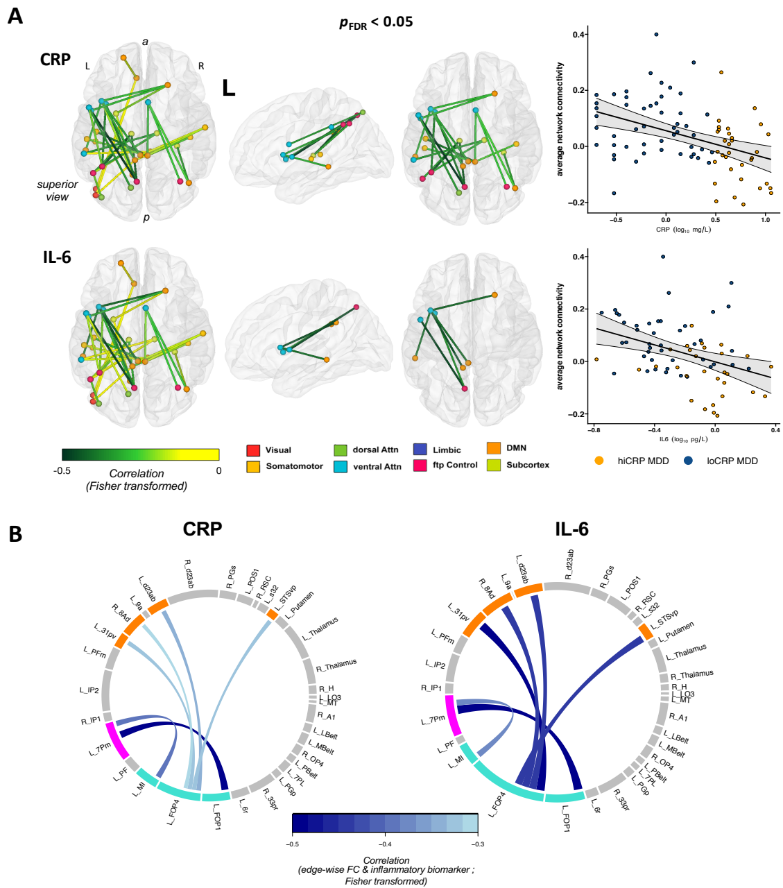
Figure 2: Functional connectivity association with inflammatory proteins in all MDD cases. (A) First column: edge-wise functional connectivity (FC) within HC vs hiCRP MDD network correlated with CRP (N=83 MDD) and IL-6 (N=72 MDD). Second column: a subset of edges had functional connectivity significantly correlated with inflammatory protein concentrations (FDR < 5%). Third column: scatterplots of the continuous relationships between average network connectivity and blood concentrations of CRP and IL-6 with the best-fitting regression lines shown with 95% confidence intervals band. (B) Strength of correlation between edge-wise FC and blood concentrations of CRP and IL-6 are denoted by intensity of blue colouration and link thickness. Only edges with attenuated connectivity significantly related to both CRP and IL-6, surviving FDR correction are shown here. IL-6 appears to show more robust negative correlation with FC compared to CRP across all edges.
