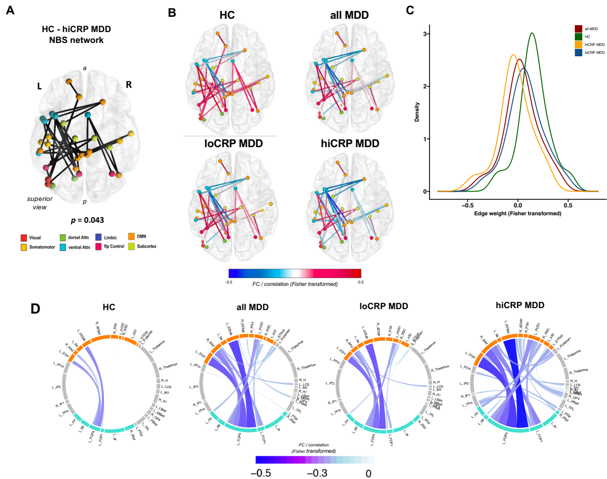
Figure 1: Network-based case-control differences in functional connectivity. (A) Network of case-control (HC vs hiCRP MDD) FC differences – modelling composite effect of inflammation and depression – identified by Network Based Statistics (NBS). A network comprising 38 edges or connections, across 33 nodes or regions, was generated by testing a one-tailed hypothesis, i.e. HC > hiCRP MDD, and reported here at the highest primary threshold t_{primary}=3.8 , at which a significant ( P<0.05 ) network was identifiable. (B) Group-averaged functional connectivity across this case-control network, plotted for each group. Across HC, loCRP MDD and hiCRP MDD, reduced functional connectivity (FC) was observed (more blue edges). These edges were mainly coupling default mode network (DMN)-ventral attentional (VA) functional modules, and anatomically, the insular/frontal-operculum and posterior cingulate cortical regions. (C) Distribution of edge-weights within the HC vs hiCRP MDD NBS network per group. (D) Distribution of negative edges within the HC vs hiCRP MDD NBS network across groups, visualized in topological space via radial network diagram. The outer track is divided into sectors, each denoting a node within the NBS network. Width of the sector denotes approximate weighted nodal degree i.e. the greater the number of (negative) connections, the longer the sector. Thickness and colour of links denote the strength of functional connectivity (FC), where edges with more negative FC have thicker and bluer links. Links within each sector are ordered clockwise with increasing FC. Across HC, loCRP MDD and hiCRP MDD groups, increases in both number and weight of negative edges were observed, especially between the DMN and VA functional modules.
