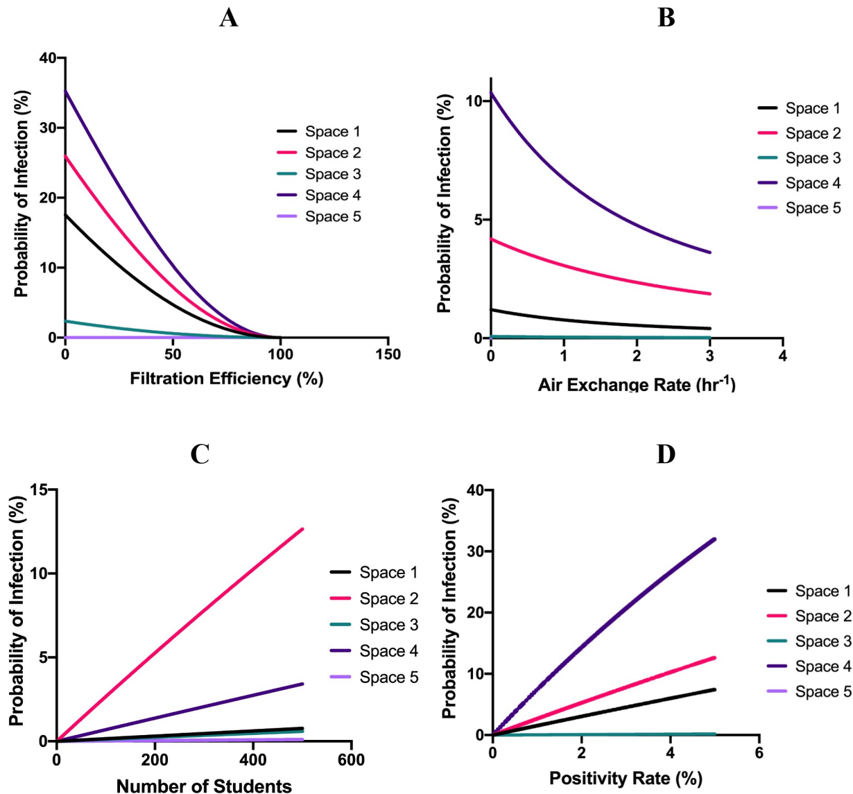
Figure 3: Relationships between dominant parameters in the model and probability of infection in five generic university spaces. A - Mask Filtration Efficiency vs. Probability of Infection, assuming constant values for all other parameters (i.e., positivity rate, room volume, air exchange rate, normal room capacity, time per visit, and total number of visits per semester) in each generic space. B - Air Exchange Rate vs. Probability of Infection, assuming the same constant values for all other parameters in each generic space. C - Number of Students vs. Probability of Infection, assuming the same constant values for all other parameters in each generic space. D - Positivity Rate vs. Probability of Infection, assuming the same constant values for all other parameters in each generic space. (See S1 Table for details on these parameters for these five generic spaces).
