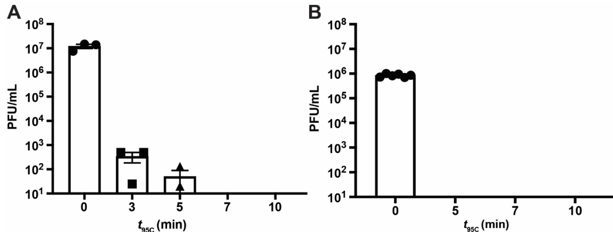
Figure 2. 95 °C heat-inactivation durations and subsequent SARS-CoV-2 virus infectivity. Plaque-forming units (PFU) per mL after 95 °C heat inactivation of infectious SARS-CoV-2 for no heating (solid black circles) and 3 (solid black squares), 5 (solid black upright triangles) min in (A) viral growth media and (B) human saliva. All data represent the mean of triplicate samples +/- SEM.
