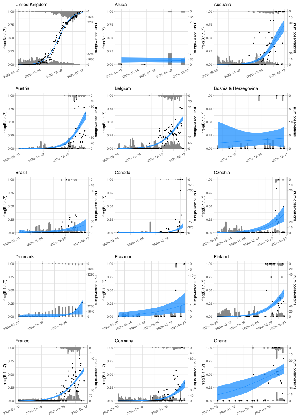
Figure S6: Fits from the population genetic model to the daily variant data for B.1.1.7. Gray bars show histograms of numbers of observations of B.1.1.7 (upper axis) and all other variants (lower axis) each day. Black dots are the daily frequencies. Blue shows the frequencies predicted from the model, with 95% credible intervals shaded.
