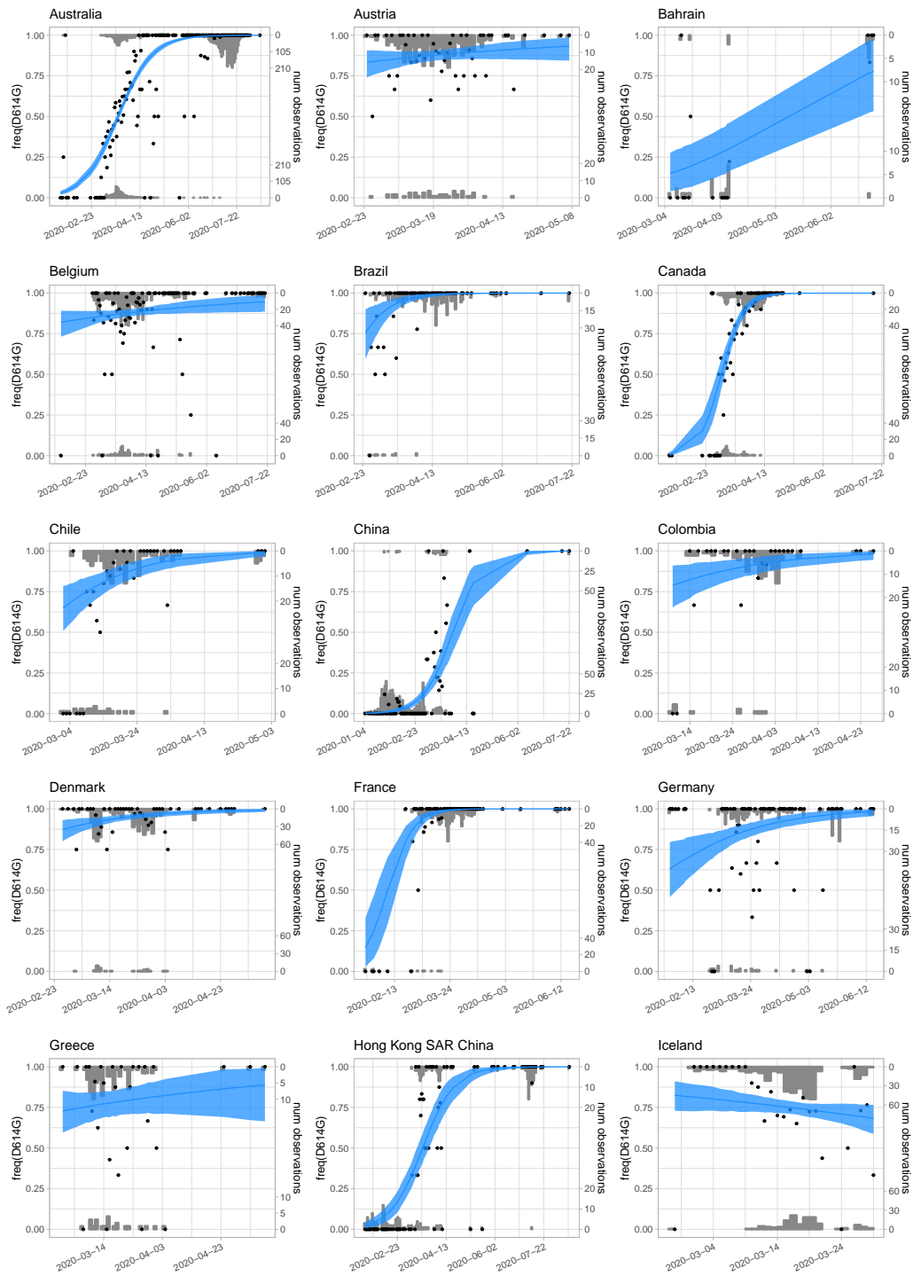
Figure S5: Fits from the population genetic model to the daily variant data for D614G. Gray bars show histograms of numbers of observations of D614G (upper axis) and all other variants (lower axis) each day. Black dots are the daily frequencies. Blue shows the frequencies predicted from the model, with 95% credible intervals shaded.
