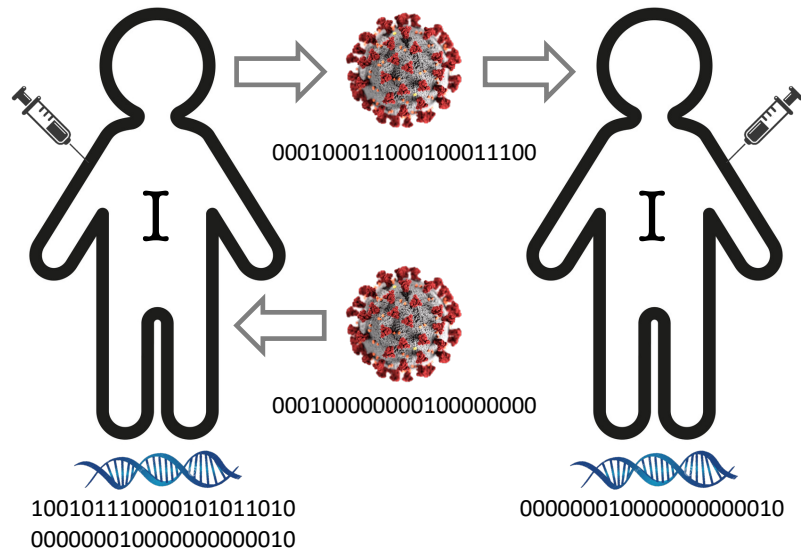
Fig S20 | Viral transmission and evolution of vaccine escape in a population of vaccinated hosts. Same as Fig S19, but here the host on the left is either: 1) vaccinated while infected, or 2) treated with immunologically similar monoclonal antibodies while infected. In either case, the virus will infect the unprotected host prior to vaccination or antibody therapy. The subsequent administration of vaccination or antibody therapy will then have the effect of creating soft selection for vaccine escape mutants in an already large within-host viral population. This is a recipe for the facile evolution of vaccine escape. When the escape mutant is then passed on to the next vaccinated host, it is likely to infect that host despite being vaccinated.
