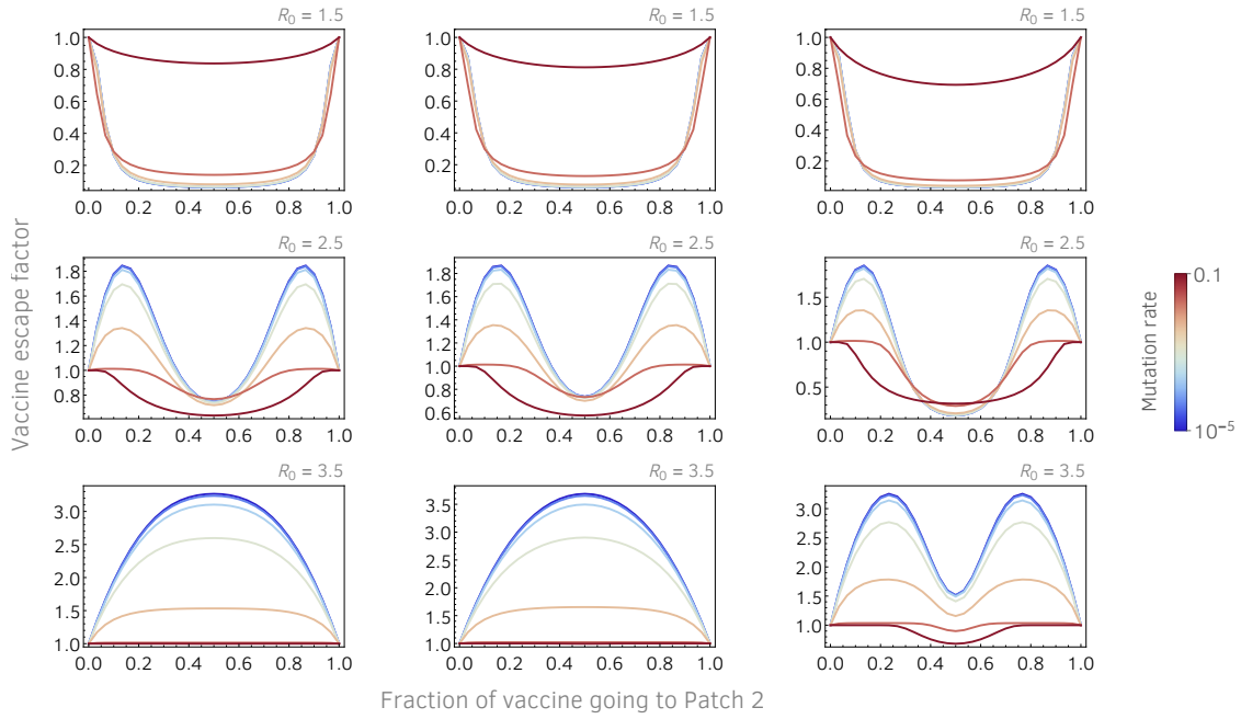
Fig S9 | Vaccine escape factor, Eq (5), as a function the fraction of vaccine that goes to Patch 2. Vaccine escape factor is defined as vaccine escape probability divided by the escape probability when all vaccine goes to one of the two patches (maximum disparity). Parameters are: \gamma = 0.1 , \lambda = 0.05 , N = 10^3 . Left-hand column: V(0) = 0 , \phi_1 + \phi_2 = 0.05 . Middle column: V(0) = 0.2 , \phi_1 + \phi_2 = 0.02 . Right-hand column: V(0) = 0.6 , \phi_1 + \phi_2 = 0.01 .
