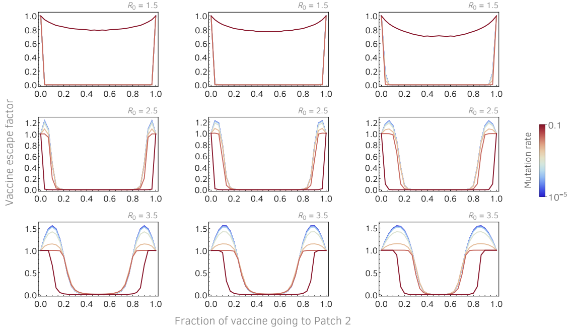
Fig S6 | Vaccine escape factor, Eq (5), as a function the fraction of vaccine that goes to Patch 2. Vaccine escape factor is defined as vaccine escape probability divided by the escape probability when all vaccine goes to one of the two patches (maximum disparity). Parameters are: \gamma = 0.1 , \lambda = 0.2 , N = 10^5 . Left-hand column: V(0) = 0 , \phi_1 + \phi_2 = 0.05 . Middle column: V(0) = 0.2 , \phi_1 + \phi_2 = 0.02 . Right-hand column: V(0) = 0.6 , \phi_1 + \phi_2 = 0.01 .
