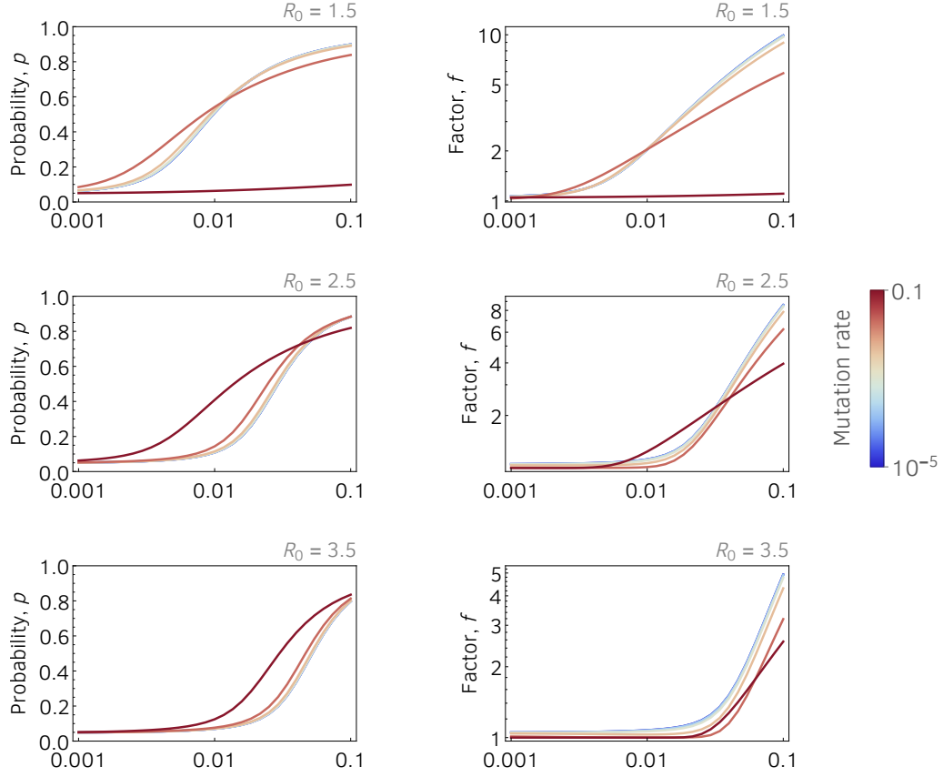
Fig S3 | Parameters are: \beta = \gamma R_0 , \gamma = 0.1 , \lambda = 0.05 , N = 10^3 .
