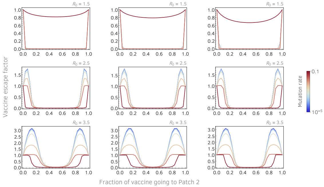
Fig S7 | Vaccine escape factor, Eq (5), as a function the fraction of vaccine that goes to Patch 2. Vaccine escape factor is defined as vaccine escape probability divided by the escape probability when all vaccine goes to one of the two patches (maximum disparity). Parameters are: \gamma = 0.1 , \lambda = 0.05 , N = 10^5 . Left-hand column: V(0) = 0 , \phi_1 + \phi_2 = 0.05 . Middle column: V(0) = 0.2 , \phi_1 + \phi_2 = 0.02 . Right-hand column: V(0) = 0.6 , \phi_1 + \phi_2 = 0.01 .
