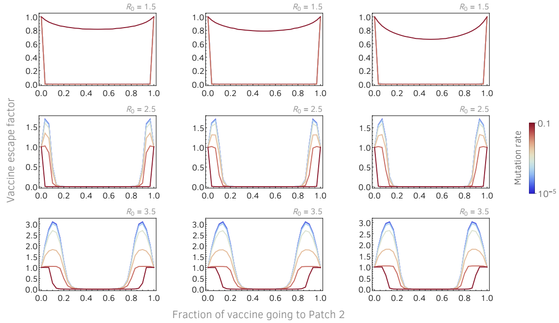
Fig S8 | Vaccine escape factor, Eq (5), as a function the fraction of vaccine that goes to Patch 2. Vaccine escape factor is defined as vaccine escape probability divided by the escape probability when all vaccine goes to one of the two patches (maximum disparity). Parameters are: \gamma = 0.1 , \lambda = 0.05 , N = 10^7 . Left-hand column: V(0) = 0 , \phi_1 + \phi_2 = 0.05 . Middle column: V(0) = 0.2 , \phi_1 + \phi_2 = 0.02 . Right-hand column: V(0) = 0.6 , \phi_1 + \phi_2 = 0.01 .
