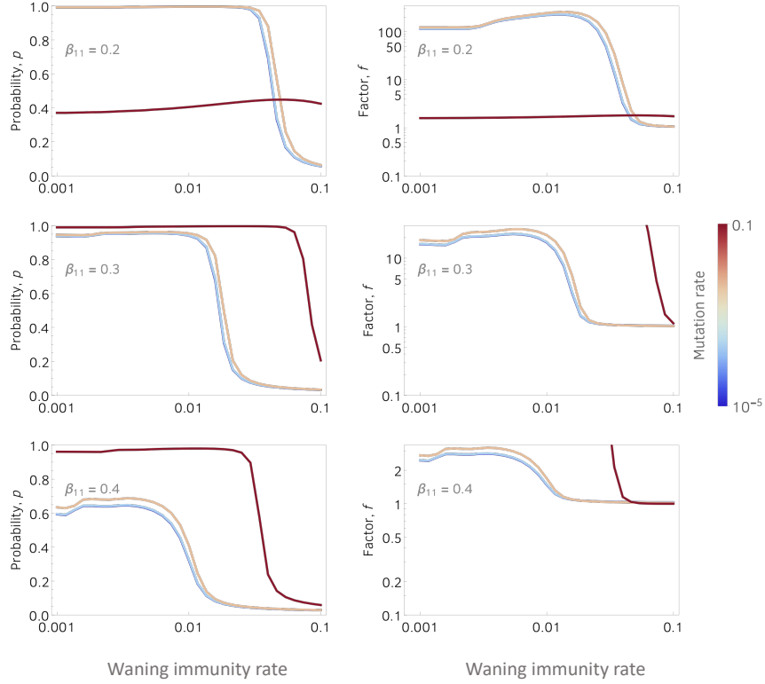
Fig S15 | Parameters are: \gamma = 0.1 , \lambda = 0.1 , \phi_1 = 0.02 , \phi_2 = 0 .
