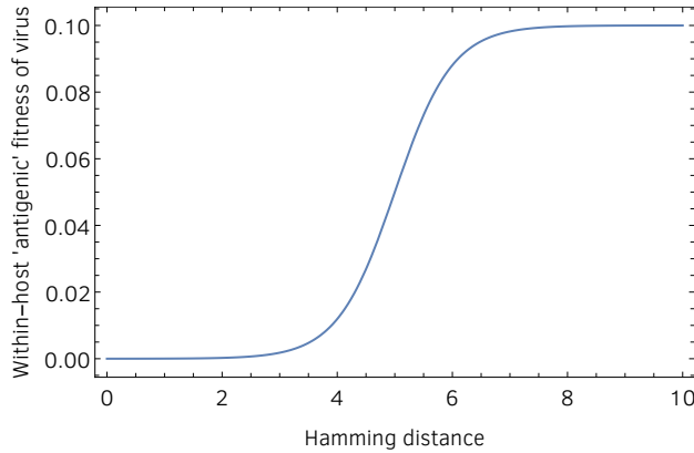
Fig S16 | Antigenic component of viral fitness as a function of the Hamming distance between the antigenic configuration of a virion and the immune configuration of its host. Because virions can have different antigenic configurations and because these configurations can undergo mutation, the viral antigenic configuration can evolve within-host to be increasingly distinct from the host’s immune configuration.
