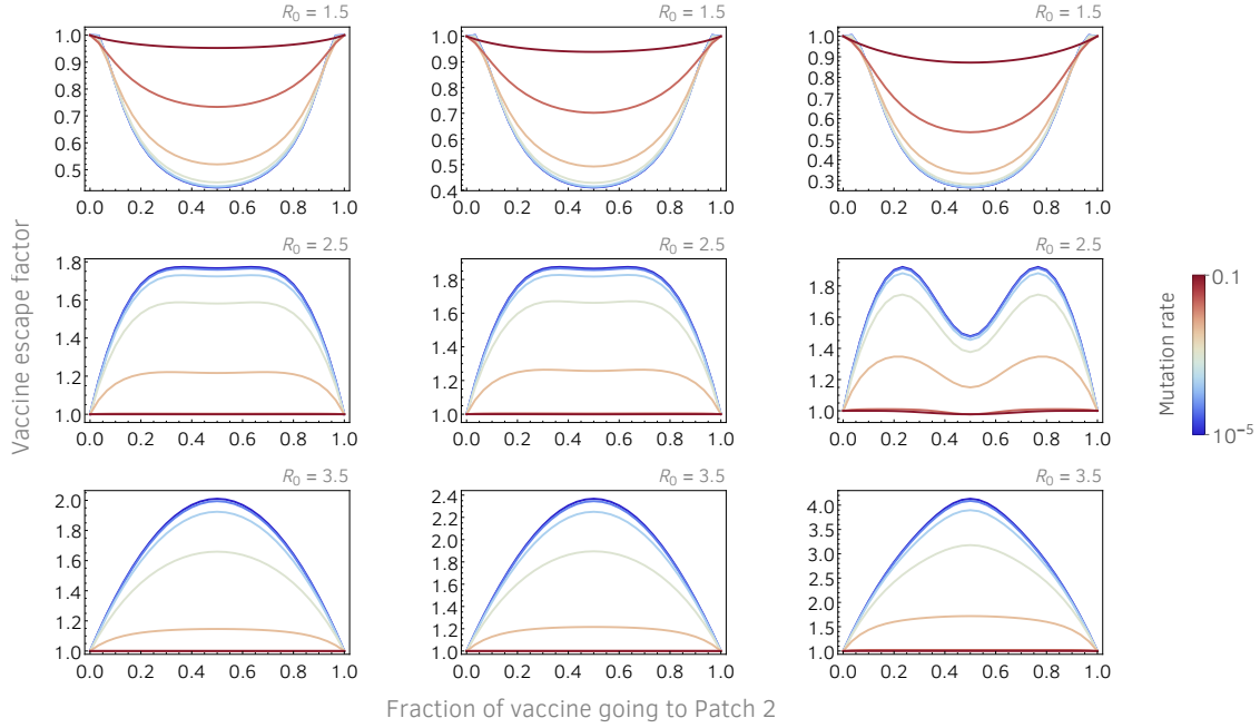
Fig S10 | Vaccine escape factor, Eq (5), as a function the fraction of vaccine that goes to Patch 2. Vaccine escape factor is defined as vaccine escape probability divided by the escape probability when all vaccine goes to one of the two patches (maximum disparity). Parameters are: \gamma = 0.1 , \lambda = 0.05 , N = 10^2 . Left-hand column : V(0) = 0 , \phi_1 + \phi_2 = 0.05 . Middle column : V(0) = 0.2 , \phi_1 + \phi_2 = 0.02 . Right-hand column : V(0) = 0.6 , \phi_1 + \phi_2 = 0.01 .
