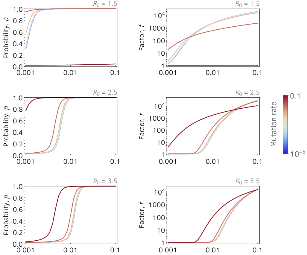
Fig S1 | Parameters are: \beta = \gamma R_0 , \gamma = 0.1 , \lambda = 0.02 , N = 10^5 .
