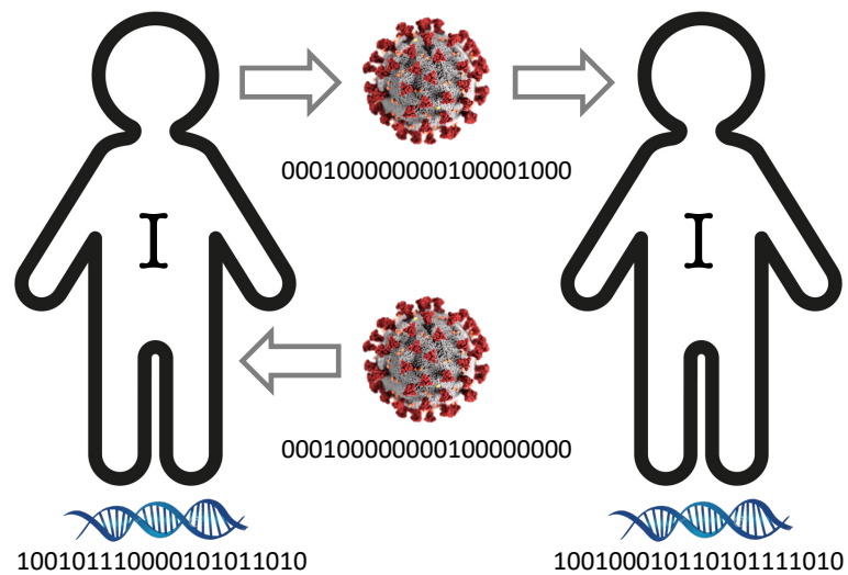
Fig S18 | Viral transmission and evolution in a population of unvaccinated hosts. The infecting virus (lower middle) has an epitope sequence very close to all zeros. It is able to infect the host on the left because the Hamming distance between the viral epitope (sequence below infecting virus) and host antibody (sequence on lower left) is large, so the host's immune system does not recognize the virus. The host on the left then transmits a slightly mutated virus (upper middle) to the host on the right. Again, this secondary infection is possible because the Hamming distance between the viral epitope (sequence below transmitted virus) and host antibody (sequence on lower right) is large, so the host's immune system does not recognize the virus.
