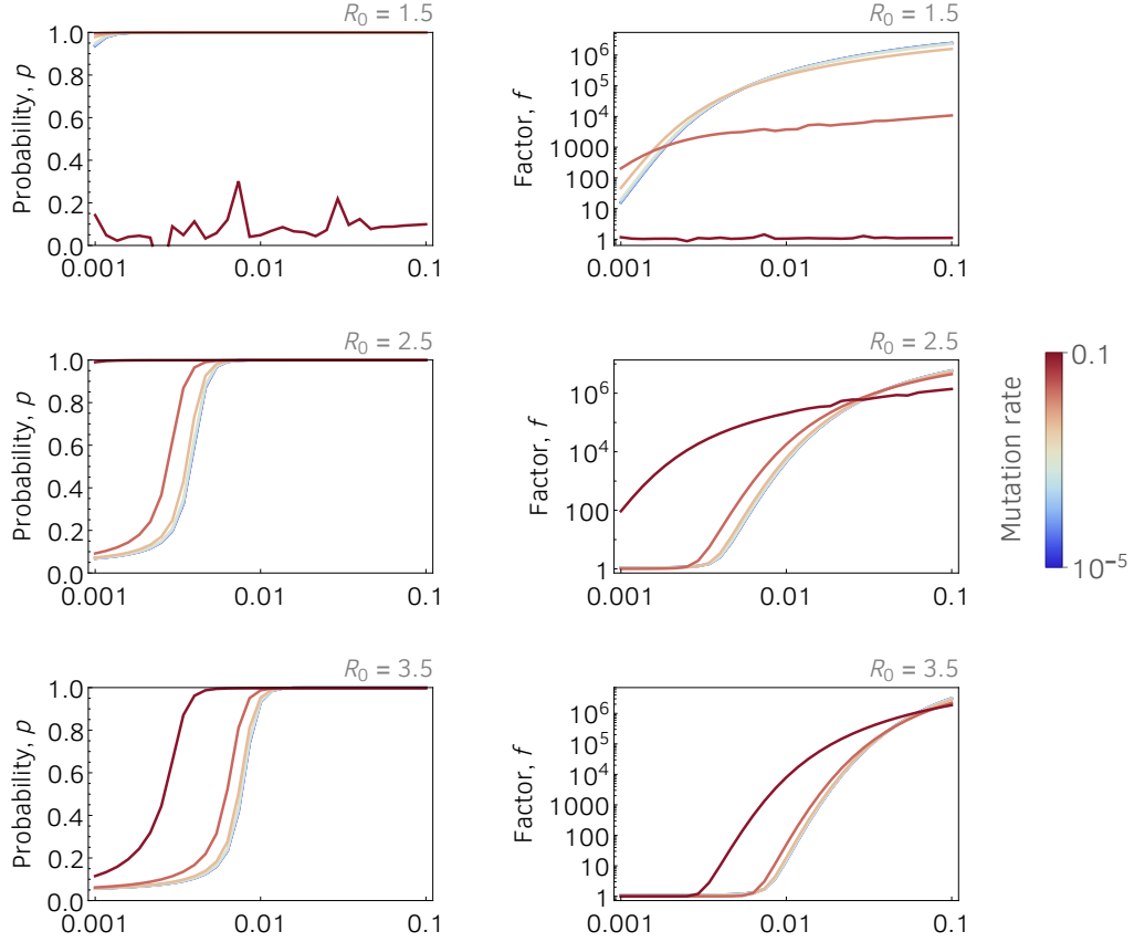
Fig S4 | Parameters are: \beta = \gamma R_0 , \gamma = 0.1 , \lambda = 0.05 , N = 10^7 .
