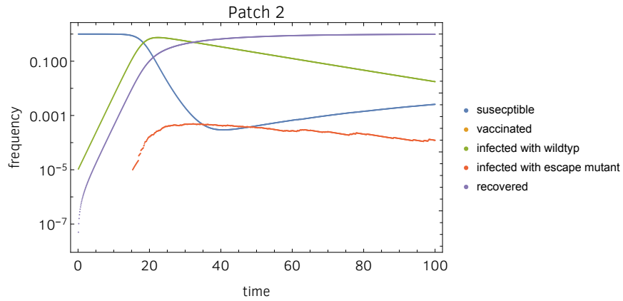
Fig S13 | Dynamics of epidemic in Patch 2. We plot a representative simulation. Escape mutant arose in Patch 2 and migrated to Patch 1 at generation 34.5, as indicated in Fig S11
