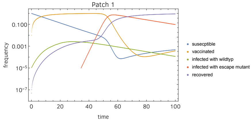
Fig S12 | Dynamics of epidemic in Patch 1. We plot a representative simulation. Escape mutant arose in Patch 2 and migrated to Patch 1 at generation 34.5, as indicated in Fig S11
