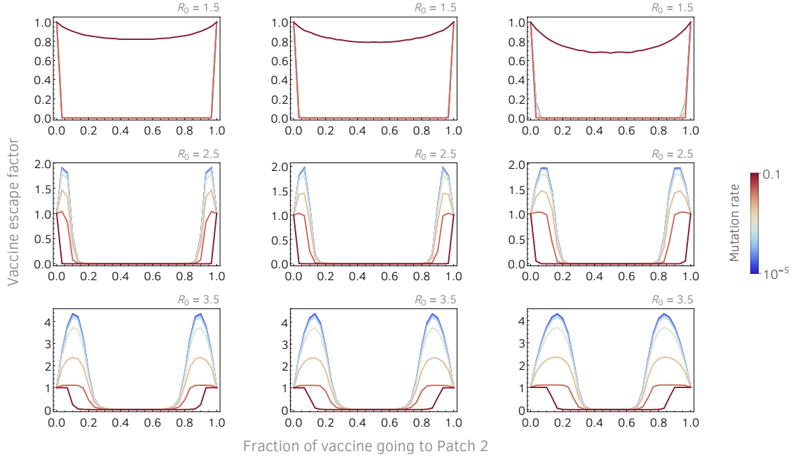
Fig S5 | Vaccine escape factor, Eq (5), as a function the fraction of vaccine that goes to Patch 2. Vaccine escape factor is defined as vaccine escape probability divided by the escape probability when all vaccine goes to one of the two patches (maximum disparity). Parameters are: \gamma = 0.1 , \lambda = 0.02 , N = 10^5 . Left-hand column: V(0) = 0 , \phi_1 + \phi_2 = 0.05 . Middle column: V(0) = 0.2 , \phi_1 + \phi_2 = 0.02 . Right-hand column: V(0) = 0.6 , \phi_1 + \phi_2 = 0.01 .
