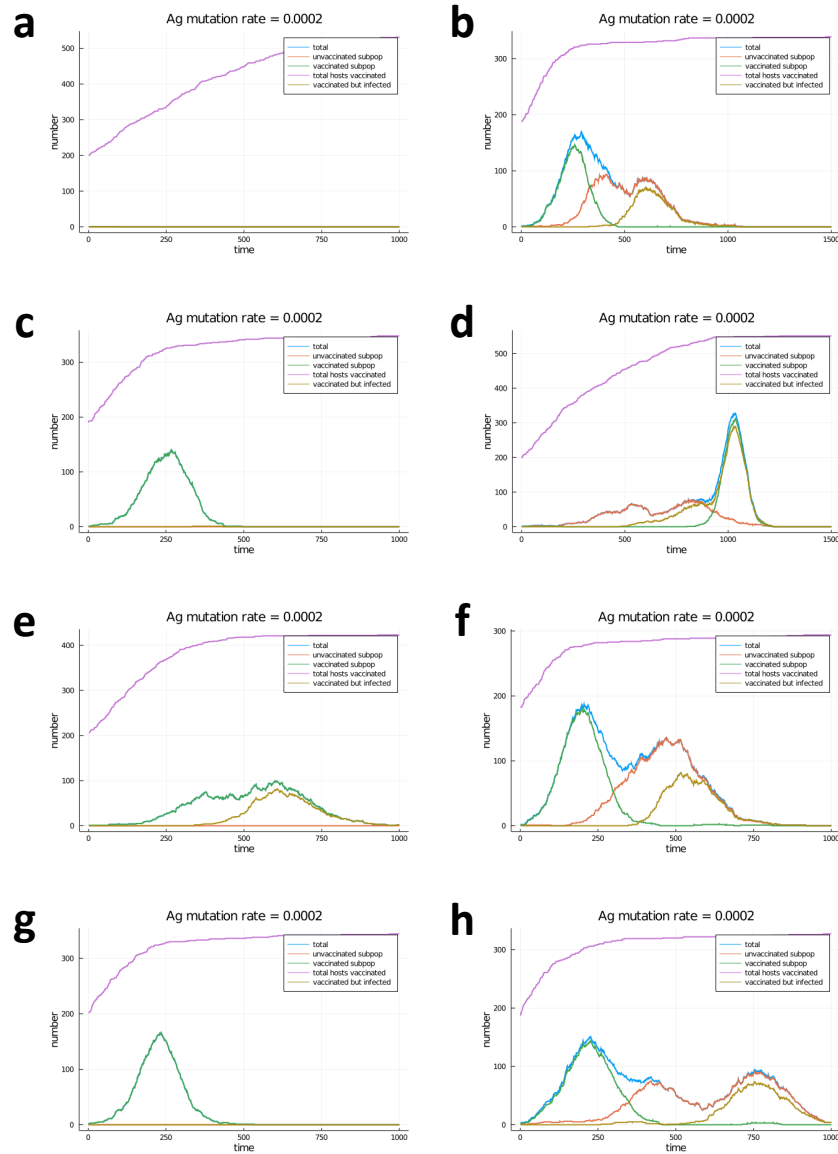
Fig S21 | Comparing one- and two-compartment simulations. Plots on the left derive from simulations with only one compartment with vaccination. Plots on the right derive from simulations with two compartments of equal size: one with vaccination and one with no vaccination. There was a low rate of migration between the two compartments. All simulations started out with a single infected host in each compartment and had exactly the same parameters. The green curve is number infected in the compartment with vaccination. The red curve is the number infected in the compartment with no vaccination. The blue curve is the total number infected. The purple curve is total number of hosts vaccinated (in the compartment with vaccination). Finally, the curve to pay special attention to is the gold-colored curve; this is the total number of hosts that are both vaccinated and infected; this is the indicator of how much vaccine escape there is. With the exception of plot e , vaccine escape does not appear in the simulations with a single vaccinated compartment (plots on left); however, significant vaccine escape appears in the simulations with one vaccinated compartment and one unvaccinated compartment (plots on right).
