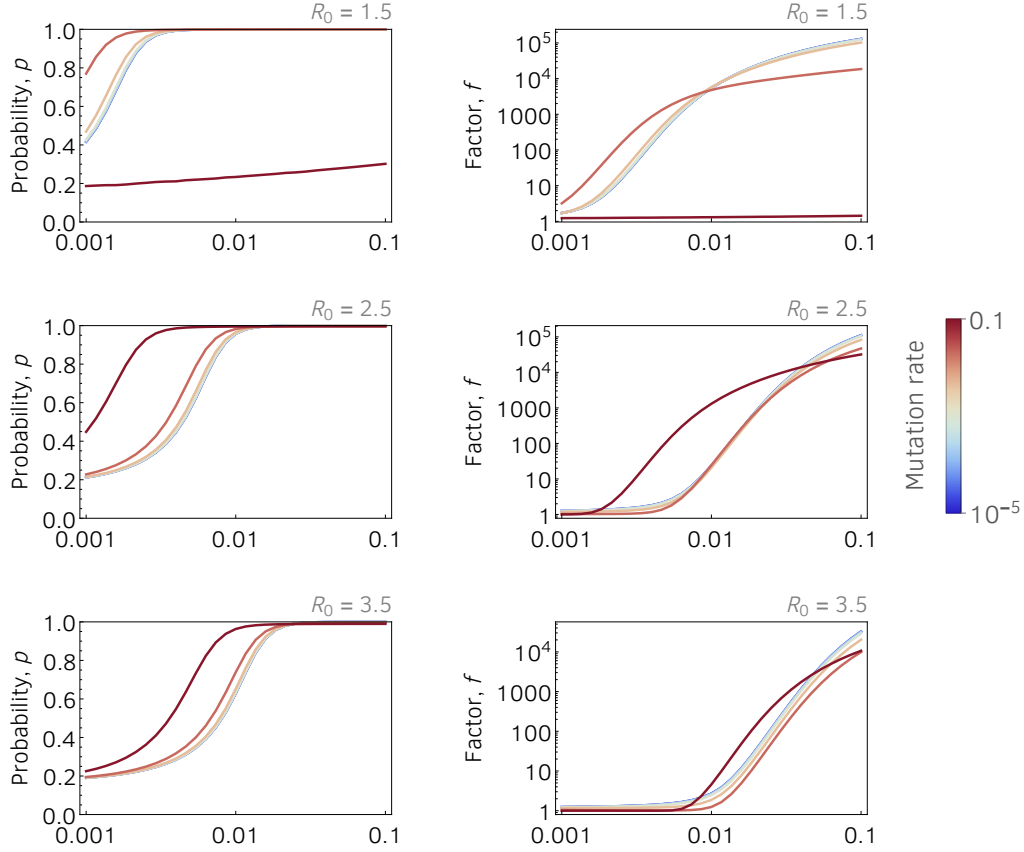
Fig S2 | Parameters are: \beta = \gamma R_0 , \gamma = 0.1 , \lambda = 0.2 , N = 10^5 .
