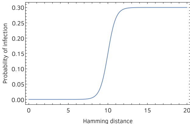
Fig S17 | Probability of infection as a function of the Hamming distance between the consensus viral epitope sequence in the inoculum and the immune antibody sequence.
