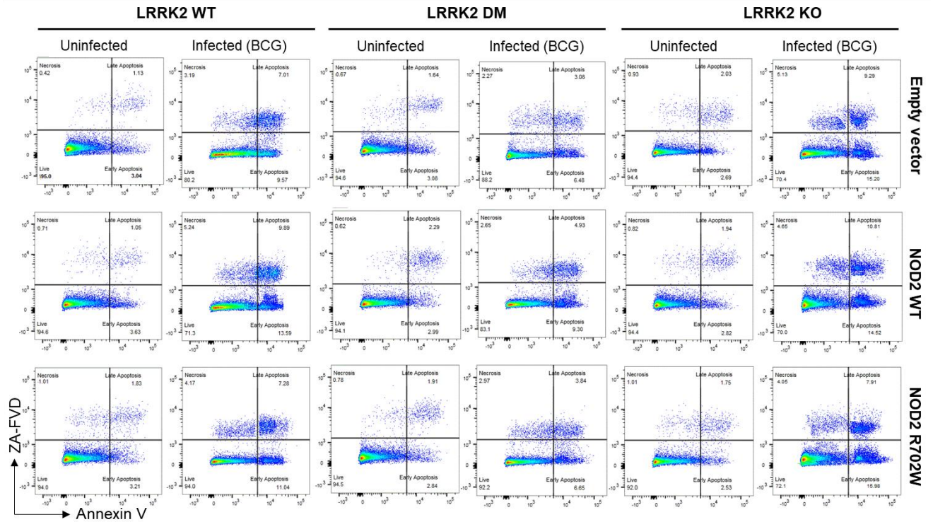
Fig. S4. Flow cytometry of the BCG-induced apoptosis analysis of NOD2-transfected cells with different LRRK2 genotypes. LRRK2 Wild-type (WT), CRISPR/Cas-edited LRRK2 double-mutant (DM, N551K+R1398H) and LRRK2 knock-out (KO) RAW264.7 cell lines were transfected with plasmids expressing NOD2 WT, NOD2 mutant (R702W) or an empty vector [pcDNA3.1+/C-(K)DYK] as a control. Twenty-four hours post-transfection, cells were left uninfected or infected with live bacillus Calmette–Guérin (BCG)-Russia (MOI 10:1) for another 24 hours. Cells were then harvested, stained with Annexin V/ZA-FVD, and analyzed by flow cytometry for apoptosis. The illustrated result is a representative of two independent experiments with similar results (done in triplicates).
