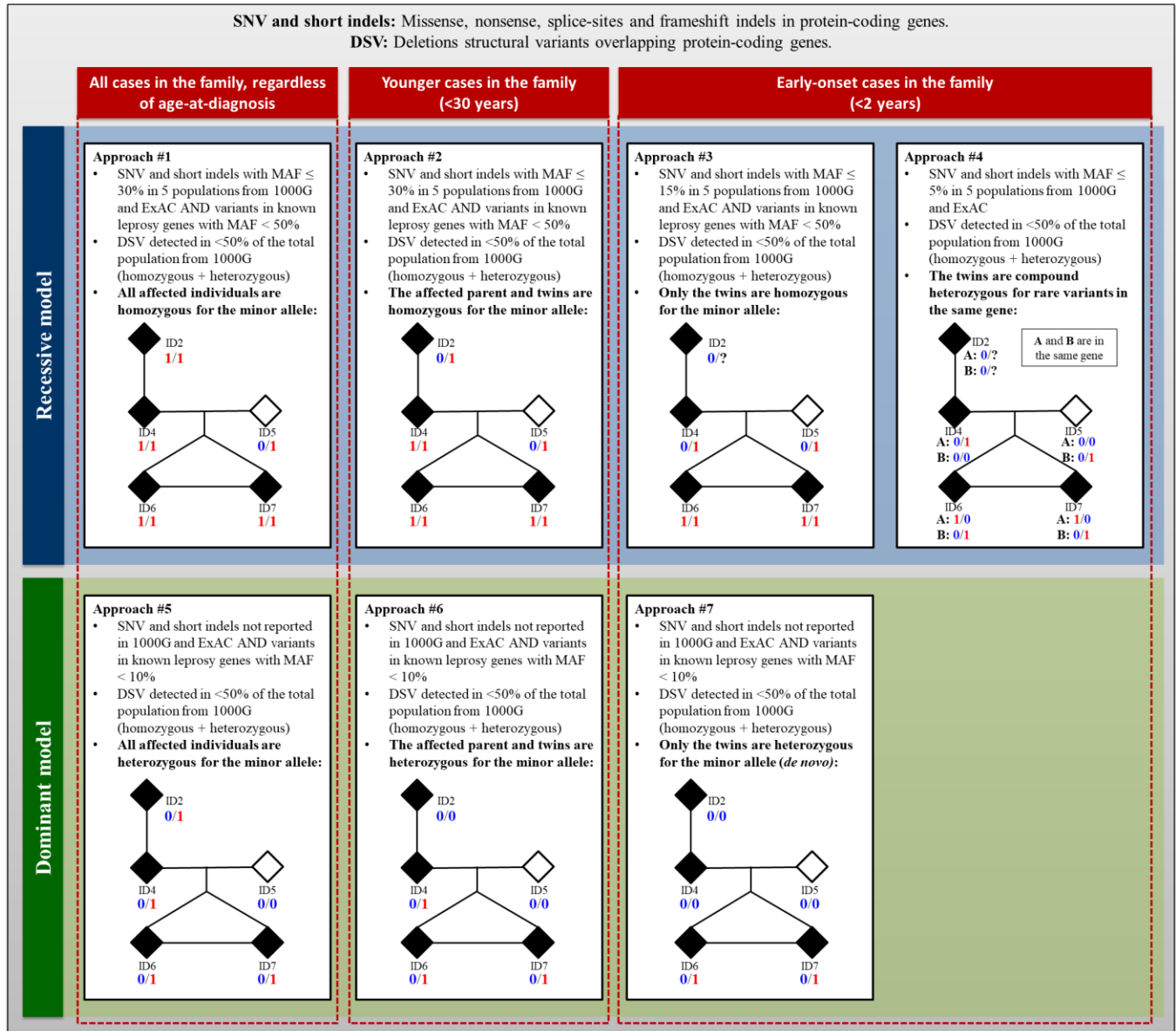
Fig. S1. Custom filtering approaches for candidate variants identification from WGS data in the studied family. First, variants were selected based on their location and impact in protein-coding genes (shown on top). Then, seven different filtering approaches were applied (approaches #1 to #7). These filtering steps were based i) on the variant frequencies in public databases, ii) on the model of inheritance and iii) on the age-at-diagnosis of the leprosy-affected family members. Specifically, recessive (#1 to #4)
