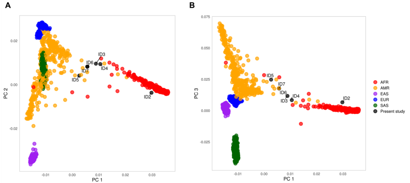
Fig. S3. Population structure of the studied family using principal component analysis based on
