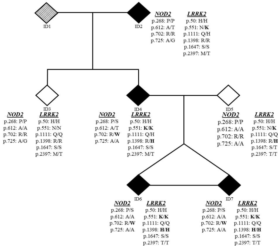
Fig. S2. All missense variants in LRRK2 and NOD2 genes detected by WGS in the studied family.
