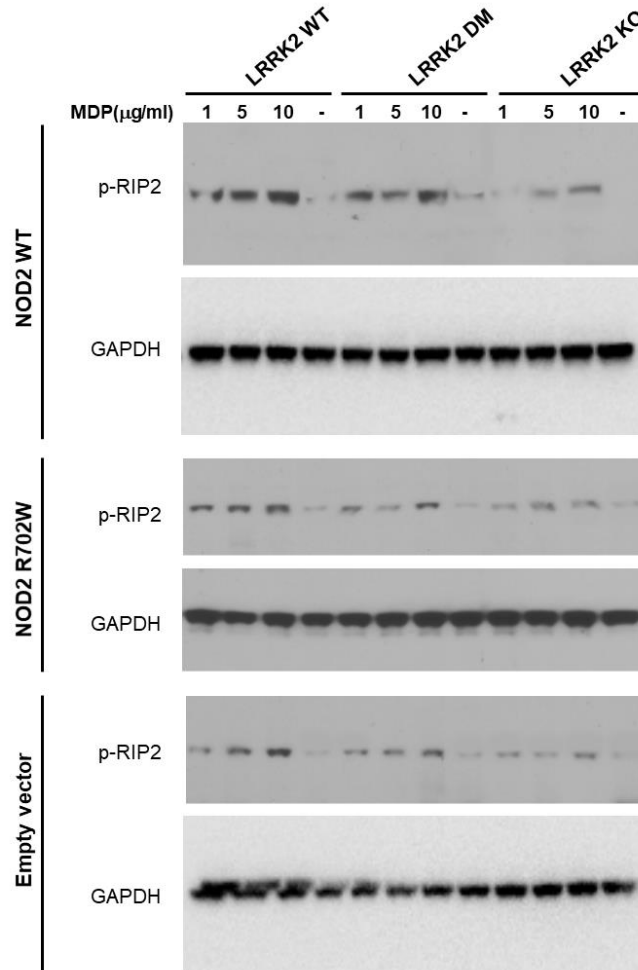
Fig. S6. Effects of LRRK2 variants on MDP-induced phosphorylation of RIP2 at Ser 176. LRRK2 Wild-type (WT), CRISPR/Cas-edited LRRK2 double-mutant (DM, N551K+R1398H) and LRRK2 knock-out (KO) RAW264.7 cell lines were transfected with plasmids expressing NOD2 WT, NOD2 mutant (R702W) or an empty vector [pcDNA3.1+/C-(K)DYK] as a control. Twenty-four hours post-transfection, cells were left untreated or treated with different concentrations of N-glycolyl MDP as indicated, for another 24 hours. Cell lysates were prepared and the phosphorylation of RIP2 (p-RIP2) in
