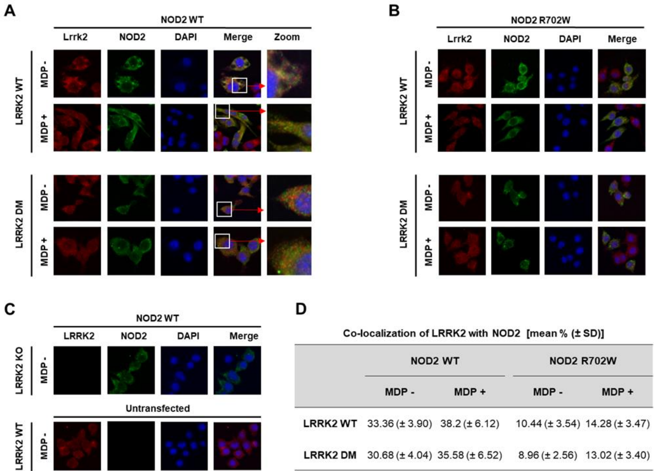
Fig. S5. Representative confocal image of colocalization of ectopically expressed NOD2 with LRRK2. Colocalization of LRRK2 wild-type (WT) and CRISPR/Cas-edited LRRK2 double-mutant (DM, N551K+R1398H) in cells transfected with plasmids expressing NOD2 WT ( A ) and NOD2 R702W ( B ). ( C ) LRRK2 KO cells (top panel) and untransfected LRRK2 WT cells (bottom panel) were used as a negative control for antibody specificity. ( A-D ) RAW264.7 cell lines with the three LRRK2 genotypes were transfected with NOD2 plasmid and a LRRK2 WT cell line was kept untransfected. Twenty-four hours after electroporation, the transfected and untransfected cells were treated with or without 10 \mu g/mL of N-glycolyl MDP for another 24 hours. Cells were fixed with 4% paraformaldehyde, permeabilized and double stained for LRRK2 and NOD2 with rabbit anti-LRRK2 (1:500) and mouse anti-FLAG (1:250) antibodies. Nuclei were stained with DAPI. Images were obtained by confocal microscopy.
