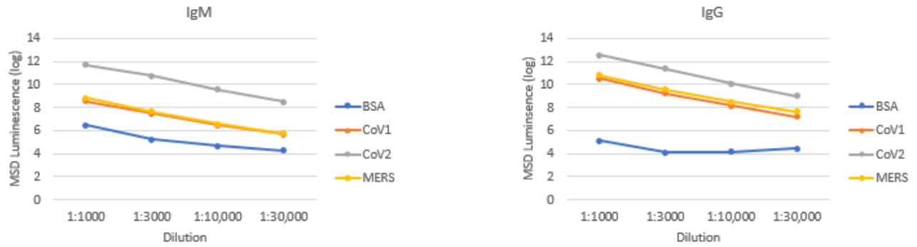
S1 Fig: Sensitivity and specificity of assay to detect SARS-CoV-2-specific antibodies. Serial dilutions (indicated on x-axis) of COVID19 patient samples (n=10) were testing for CoV-specific IgM (left panel) and IgG (right panel) in the 10-plex assay; plate antigens: BSA (negative control), spike protein of SARS CoV1, SARS-CoV-2, MERS CoV. Data expressed as mean luminescence signal (log).
