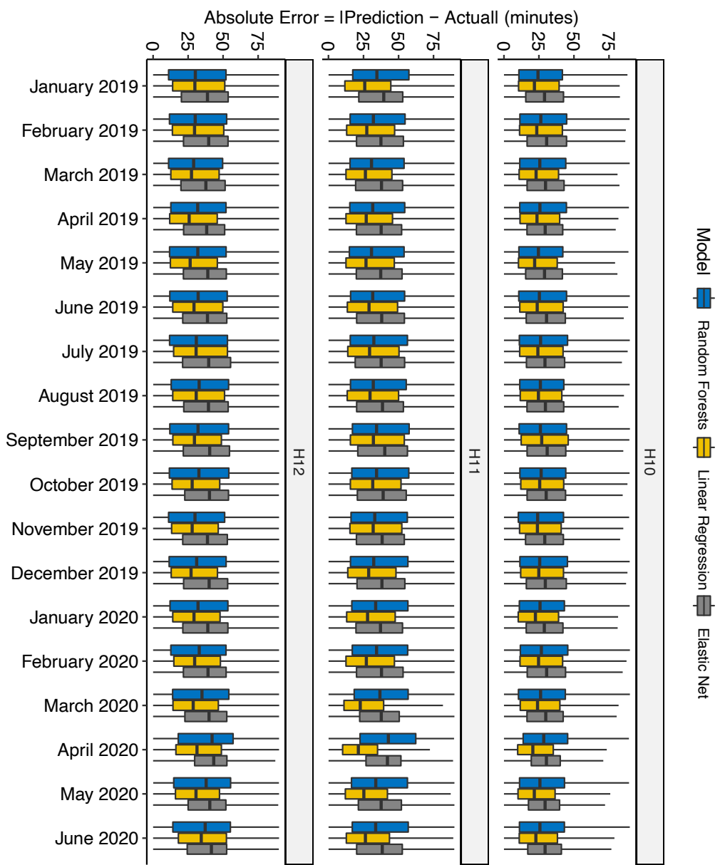
Appendix 1f. Distributions of absolute errors for wait time predictions before and during COVID19 reduced attendances in 2020
