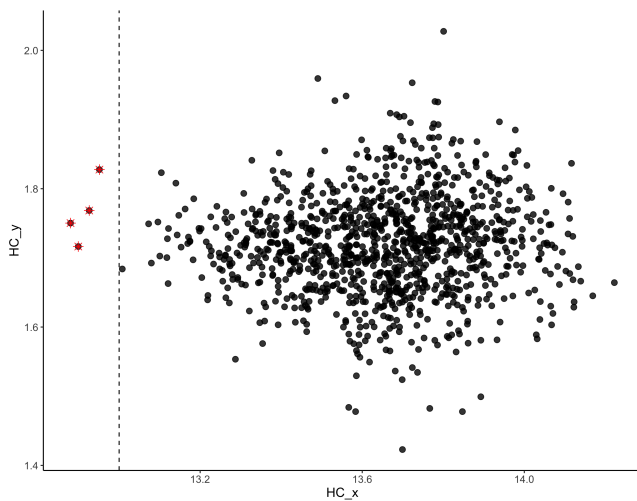
QC figure 30: Rotated HC plot based on hybridization control probes as implemented in the MethylAid package [1].
