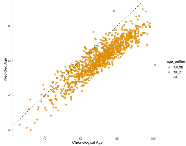
QC figure 38: Chronological age vs. Predicted Age based on the Zhang et al. age predictor [4].
