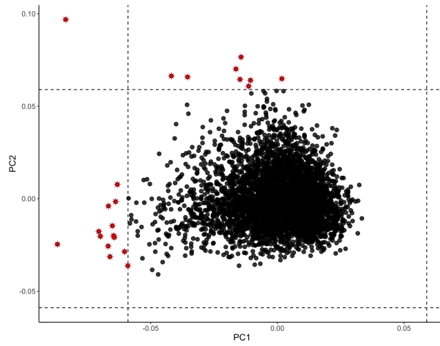
QC figure 12: Array-wide principal components, after first round of QC.
