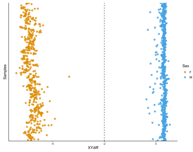
QC figure 35: Difference between median Y-chromosomal and median X-chromosomal signal intensity.
