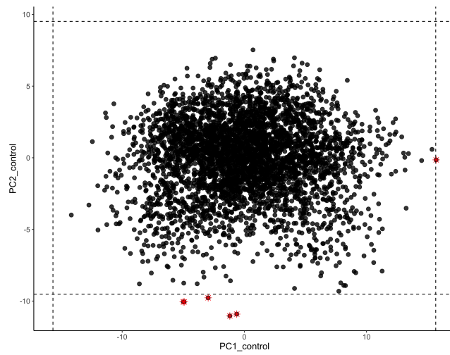
QC figure 24: Control probe principal components, after first round of QC.
