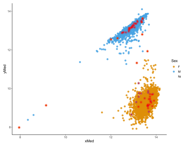
QC figure 21: Median X and Y copy number, as implemented in the minfi package [3].
