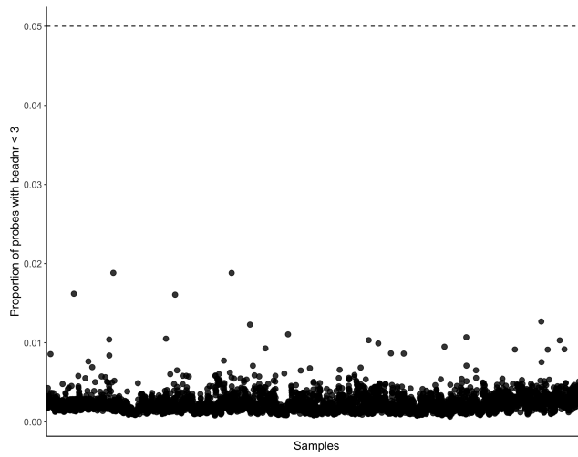
QC figure 20: Percentage of probes with beadNr < 3.
