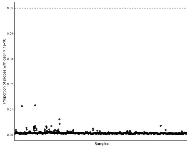
QC figure 32: Percentage of probes with detection P-value > 1 \times 10^{-16}
