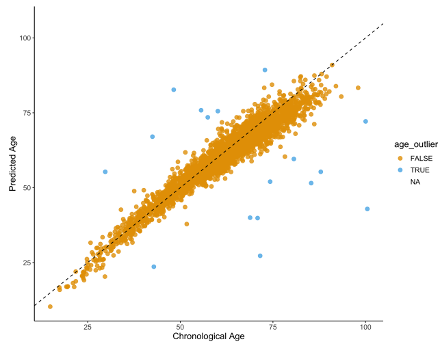
QC figure 26: Chronological age vs. Predicted Age based on the Zhang et al. age predictor [4].
