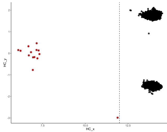
QC figure 4: Rotated HC plot based on hybridization control probes as implemented in the MethylAid package [1].
