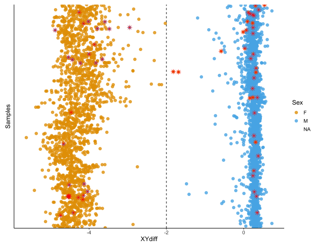
QC figure 22: Difference between median Y-chromosomal and median X-chromosomal signal intensity.
