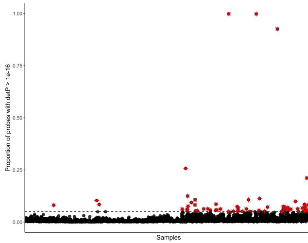
QC figure 19: Percentage of probes with detection P-value > 1 \times 10^{-16}
