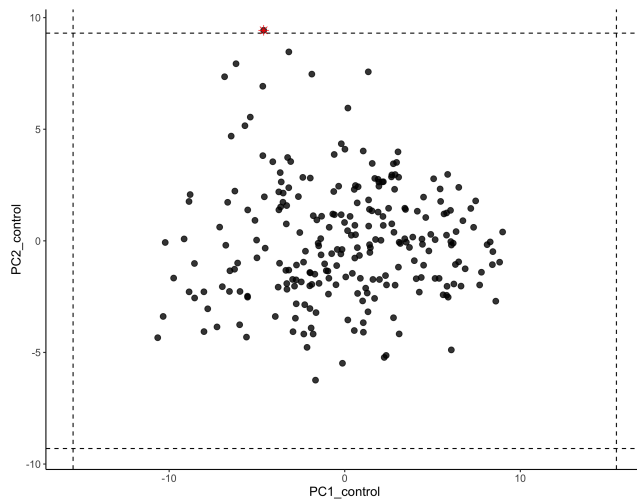
QC figure 48: Control probe principal components, after first round of QC.
