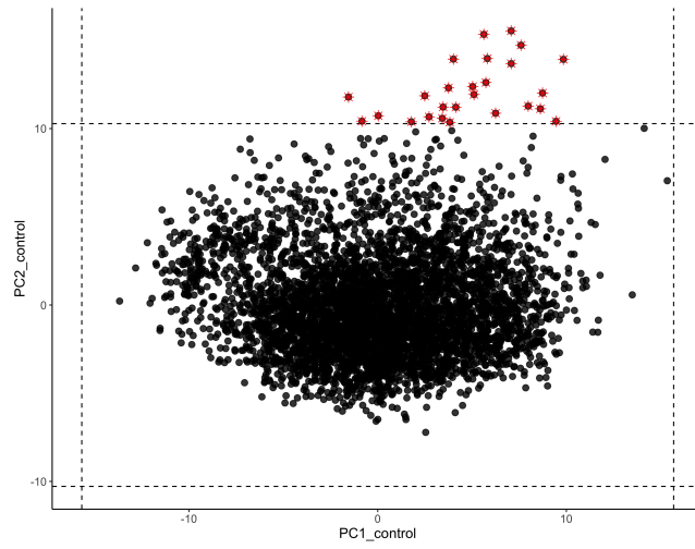
QC figure 11: Control probe principal components, after first round of QC.
