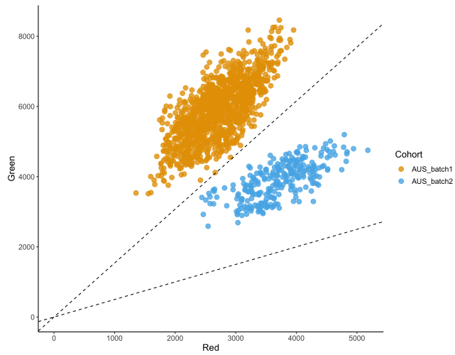
QC figure 50: Median red vs. median green signal in all Australian data, calculated in type I probes. AUS1 samples were defined based on an RG ratio <0.65 , and AUS2 samples were defined based on an RG ratio >0.65 .
