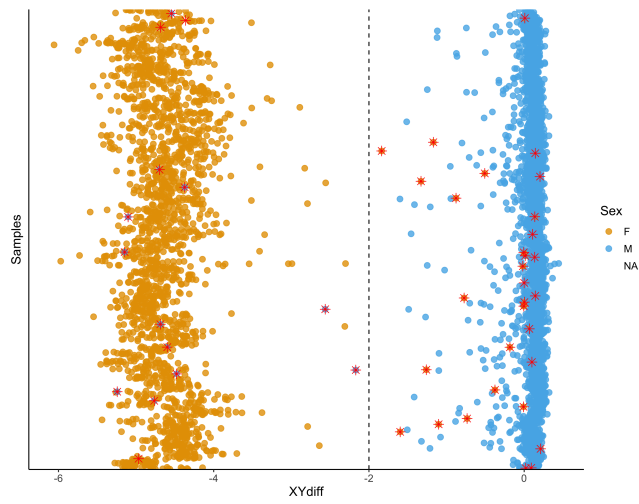
QC figure 9: Difference between median Y-chromosomal and median X-chromosomal signal intensity.
