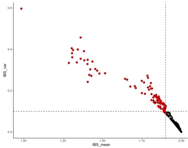
QC figure 10: Identity-by-descent (IBS) comparing DNAm-inferred SNPs and SNPs measured using whole-genome sequencing data.
