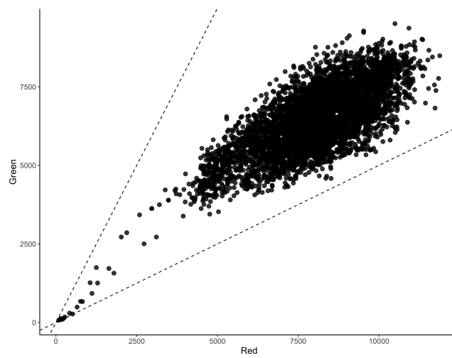
QC figure 2: Median red vs. median green signal, calculated in type I probes.
