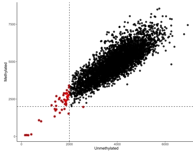
QC figure 14: Median unmethylated vs. median methylated signal.
