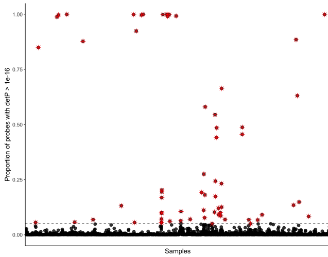
QC figure 6: Percentage of probes with detection P-value > 1 \times 10^{-16}
