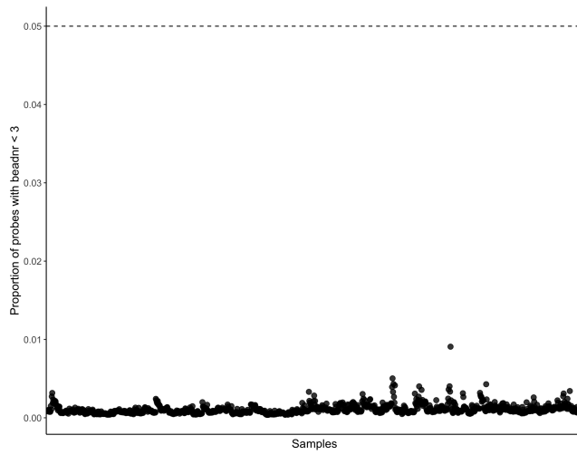
QC figure 33: Percentage of probes with beadNr < 3.
