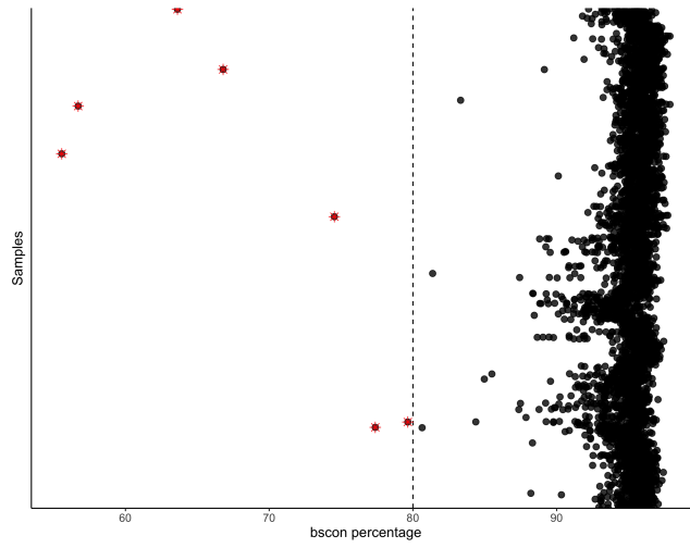
QC figure 18: bscon metric from the wateRmelon package, which measures bisulfite conversion efficiency [2].
