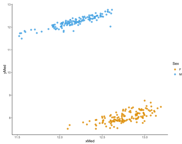
QC figure 46: Median X and Y copy number, as implemented in the minfi package [3].
