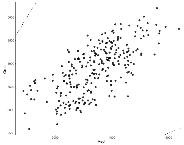
QC figure 40: Median red vs. median green signal, calculated in type I probes.
