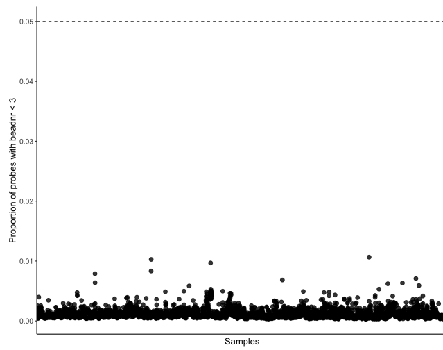
QC figure 7: Percentage of probes with beadNr < 3.
