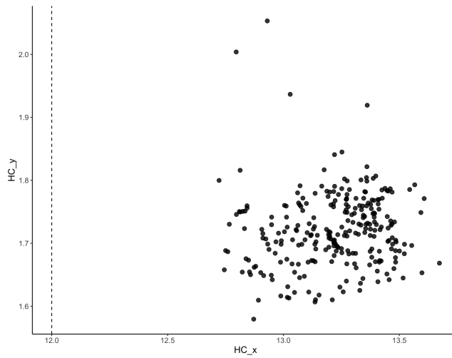
QC figure 42: Rotated HC plot based on hybridization control probes as implemented in the MethylAid package [1].
