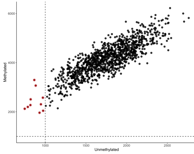
QC figure 27: Median unmethylated vs. median methylated signal.
