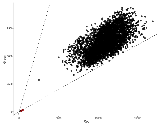
QC figure 15: Median red vs. median green signal, calculated in type I probes.
