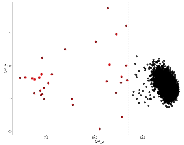
QC figure 3: Rotated OP (Overall quality) plot based on non-polymorphic control probes as implemented in the MethylAid package [1].
