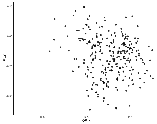
QC figure 41: Rotated OP (Overall quality) plot based on non-polymorphic control probes as implemented in the MethylAid package [1].
