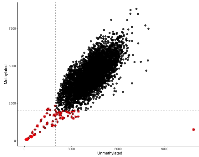
QC figure 1: Median unmethylated vs. median methylated signal.
