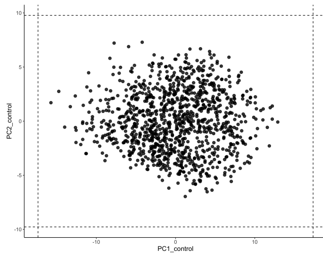
QC figure 36: Control probe principal components, after first round of QC.
