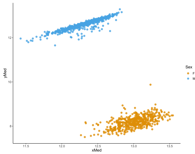
QC figure 34: Median X and Y copy number, as implemented in the minfi package [3].
