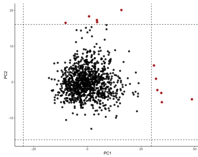
QC figure 37: Array-wide principal components, after first round of QC.
