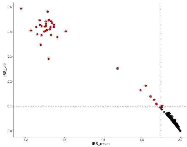
QC figure 23: Identity-by-descent (IBS) comparing DNAm-inferred SNPs and SNPs measured using whole-genome sequencing data.
