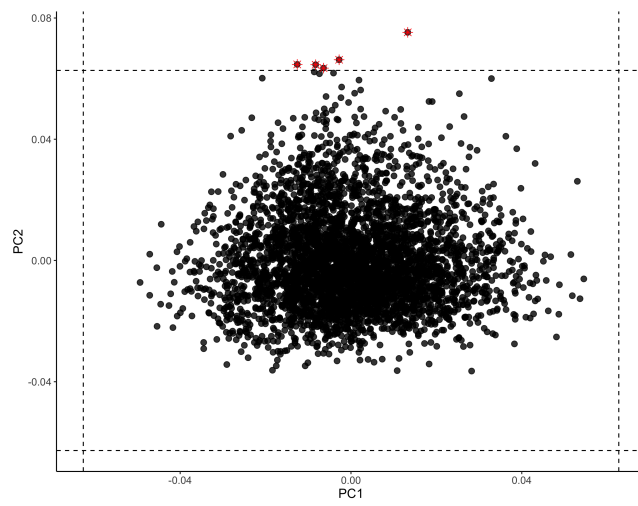
QC figure 25: Array-wide principal components, after first round of QC.
