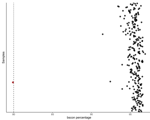
QC figure 43: bscon metric from the wateRmelon package, which measures bisulfite conversion efficiency [2].
