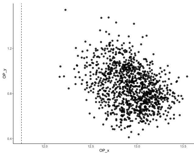
QC figure 29: Rotated OP (Overall quality) plot based on non-polymorphic control probes as implemented in the MethylAid package [1].
