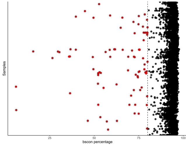
QC figure 5: bscon metric from the wateRmelon package, which measures bisulfite conversion efficiency [2].
