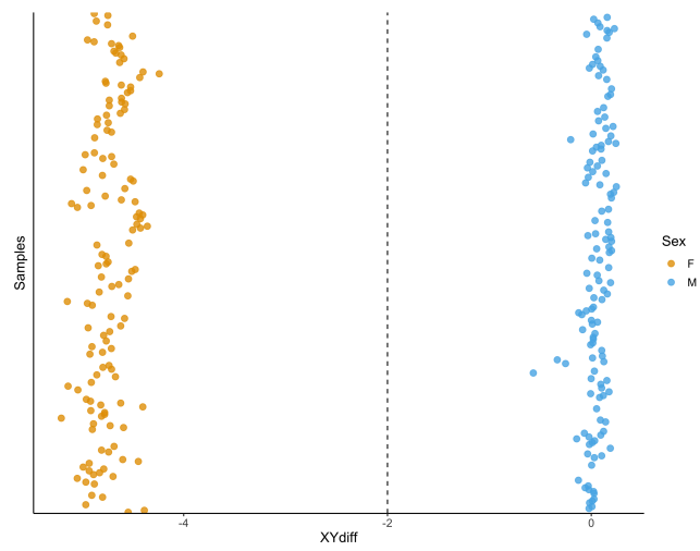
QC figure 47: Difference between median Y-chromosomal and median X-chromosomal signal intensity.
