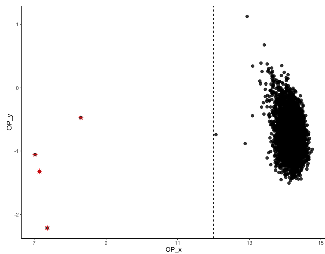
QC figure 16: Rotated OP (Overall quality) plot based on non-polymorphic control probes as implemented in the MethylAid package [1].
