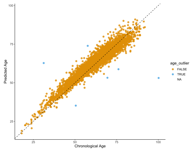
QC figure 13: Chronological age vs. Predicted Age based on the Zhang et al. age predictor [4].
