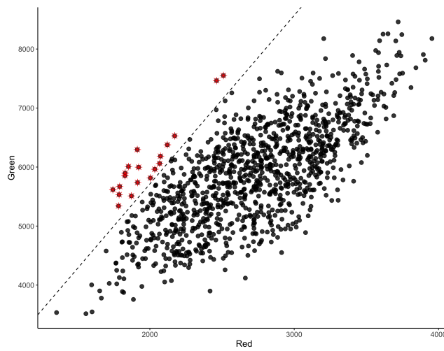
QC figure 28: Median red vs. median green signal, calculated in type I probes.
