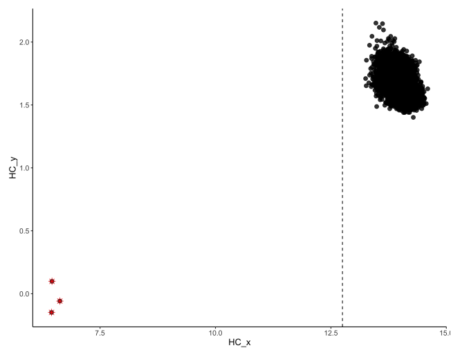
QC figure 17: Rotated HC plot based on hybridization control probes as implemented in the MethylAid package [1].
