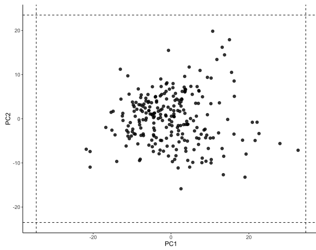
QC figure 49: Array-wide principal components, after first round of QC.
