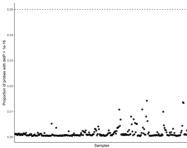
QC figure 44: Percentage of probes with detection P-value > 1 \times 10^{-16}
