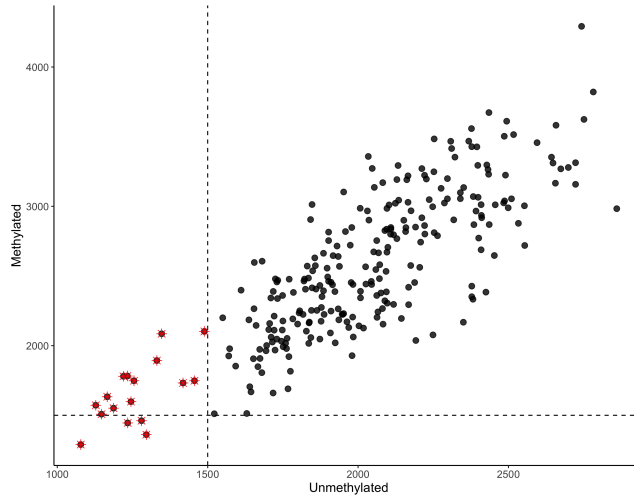
QC figure 39: Median unmethylated vs. median methylated signal.
