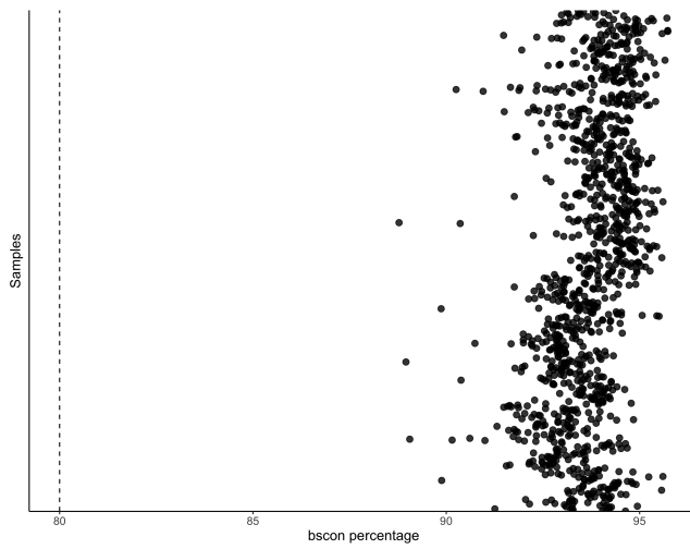
QC figure 31: bscon metric from the wateRmelon package, which measures bisulfite conversion efficiency [2].
