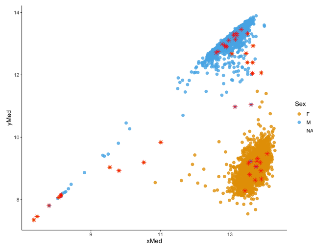
QC figure 8: Median X and Y copy number, as implemented in the minfi package [3].
