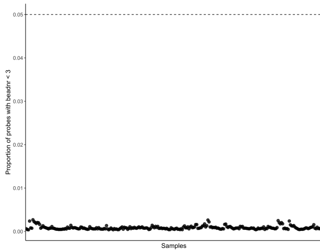
QC figure 45: Percentage of probes with beadNr < 3.
