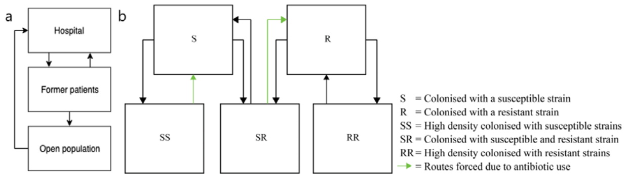
Figure 4. Compartmental model of ESBL E. coli and E. coli colonisation states
