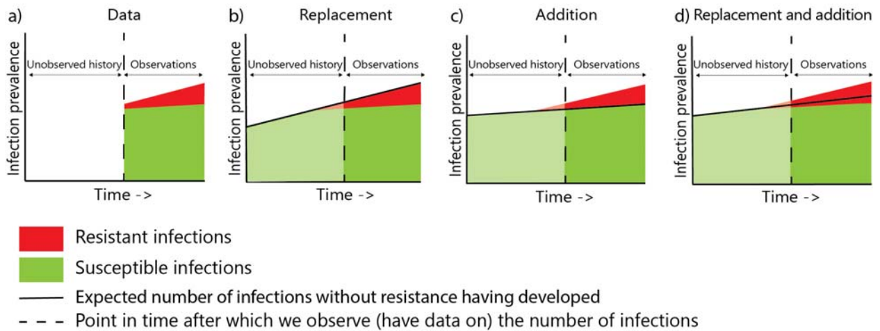
Figure 1. Three scenarios explained by addition to and replacement of susceptible infections. The observed prevalence of susceptible and resistant infections is depicted in panel a. In panel b, c and d, three potential scenarios for the prevalence in the unobserved period are depicted. Each scenario suggests a different interpretation regarding addition or replacement.
