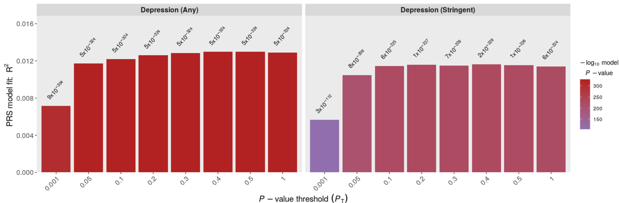
Supplementary Figure 5: Within-trait PRS - associations between PRS for MDD and depression case/control status (any/stringent) across eight P_T . Y-axis shows unadjusted R^2 (observed-scale). Note: p-value for MDD PRS predicting Depression (Any) = 0 for thresholds 0.05 to 1 due to limit on the smallest number on the R platform (5e-324).
