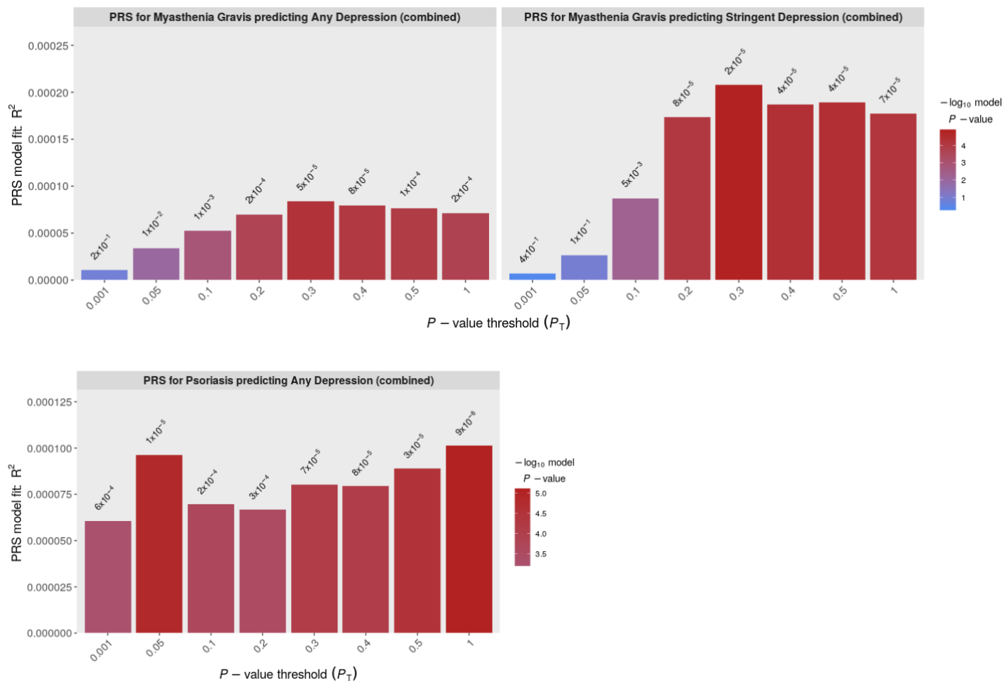
Supplementary Figure 6: Cross-trait PRS –associations between PRS for autoimmune diseases and depression case/control status (any/stringent) in men and women across eight P_T . Y-axis shows unadjusted R^2 (observed-scale). Bar charts are shown for significant results only.
