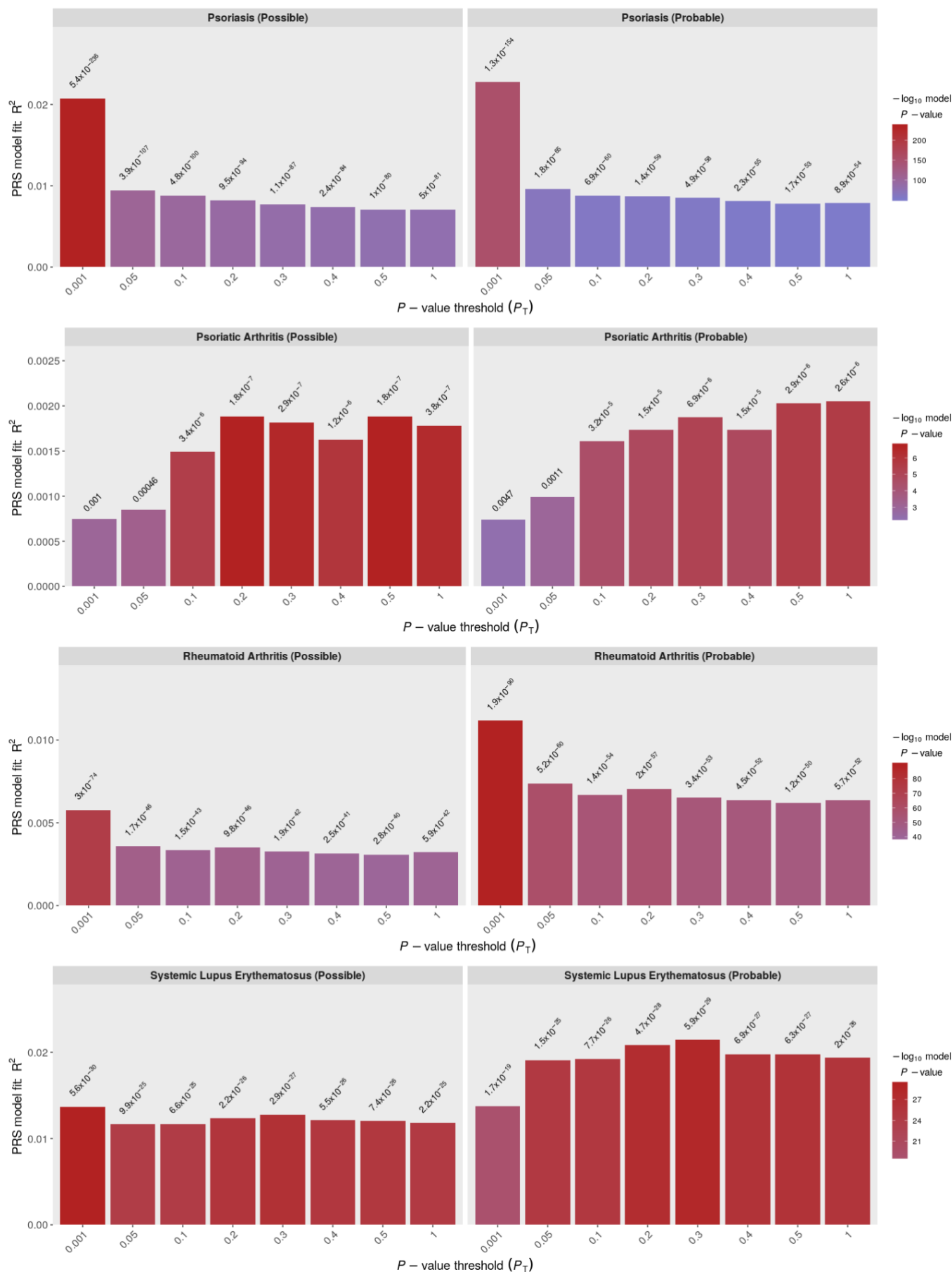
Supplementary Figure 4: Within-trait PRS - associations between PRS for autoimmune diseases and autoimmune case/control status (possible/probable) across eight P_T . Y-axis shows unadjusted R^2 (observed-scale).
